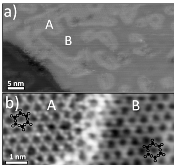
Figure 2. (a) Large scale STM image of an \text{Al}_{0.12}\text{Si}_{0.88}\text{O}_2 film. (b) High resolution STM image showing different contrast inside the islands A. The positions of the Si atoms in the top layer are shown by black circles and O atoms by open circles. (Tunneling parameters: bias 0.15 V, current 0.07 nA).
