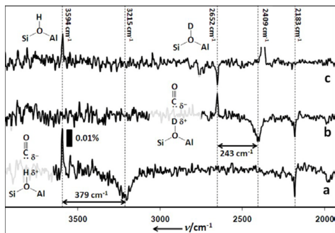
Figure 4. IRA spectra of the \text{Al}_{0.4}\text{Si}_{0.6}\text{O}_2 films, hydroxylated with \text{H}_2\text{O} (a) and \text{D}_2\text{O} (b), recorded in 2 \times 10^{-5} mbar CO ambient. The spectra were divided by reference spectra taken before CO exposure. The spectrum (c) shows the one of the OH-terminated surface upon subsequent hydroxylation with \text{D}_2\text{O} .
