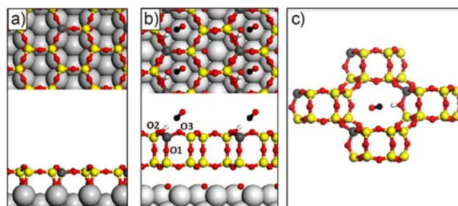
Figure 1. Structural models of an \text{AlSi}_7\text{O}_{19} film on Mo(112) (a); \text{HAlSi}_7\text{O}_{16} film on \text{O}(2\times 1)/\text{Ru}(0001) (b); and chabasite (H-CHA) with the proton on O1 (c). Top and cross views are shown in (a) and (b), adsorbed CO are shown in (b) and (c). (Note that one of the surface O atoms on Ru(0001) underneath the film is not seen in the top view). Si (yellow), O (red), Al (dark gray), C (black), H (white).
