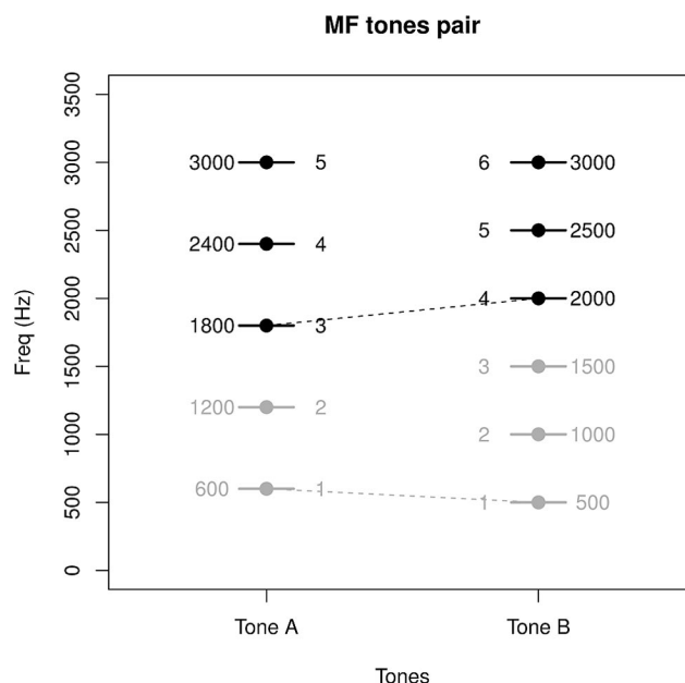
Figure 1. Basic design of missing fundamental (MF) task stimuli. Tone A (on the left) consists of three partials that could be the 3rd, 4th, and 5th harmonic of a fundamental frequency (the “first harmonic”) that is not physically present in the signal. Tone B (on the right) also consists of three partials, which could be the 4th, 5th, and 6th harmonics of a fundamental frequency (also not physically present). Crucially, the MF in Tone B is lower than that in Tone A, and the lowest frequency actually present in Tone B is higher than the lowest frequency actually present in Tone A.
