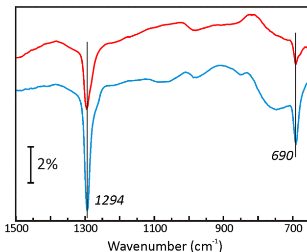
FIG. 3. IRAS-spectra of 1 MLE (top) and 2 MLE (bottom) films grown on Pt(111).
