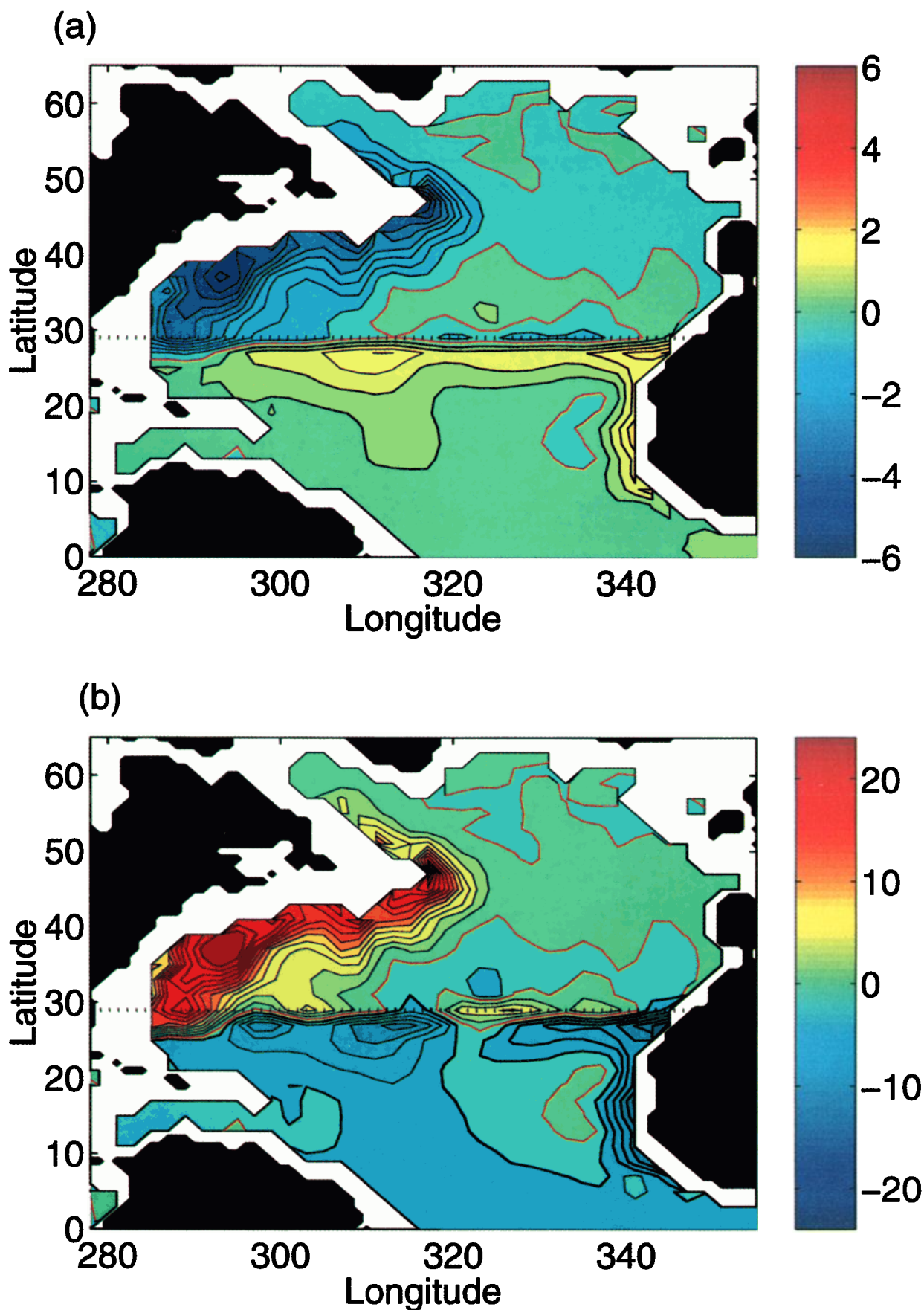
Plate 2. (a) Sensitivity of mean 1993 Atlantic heat transport across 29°N (dotted line) to temperature at 1160 m on January 1, 1993. The contour interval is 0.5 \times 10^{12} \text{ W K}^{-1} , and the zero contour is drawn in red. (b) Sensitivity of mean 1993 Atlantic heat transport across 29°N (dotted line) to salinity at 1160 m on January 1, 1993. The contour interval is 2 \times 10^{12} \text{ W (psu)}^{-1} , and the zero contour is drawn in red.
