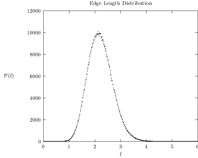
FIG. 33 A typical edge length distribution in the smooth phase for which k < k_c , or G > G_c . Note that the lattice gravitational measure of Eq. (406) cuts off the distribution at small edge lengths, while the cosmological constant term prevents large edge lengths from appearing.
