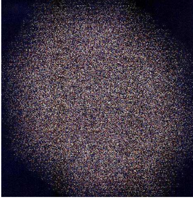
FIG. 35 Local curvatures projected on a plane, in the smooth phase G > G_c .
