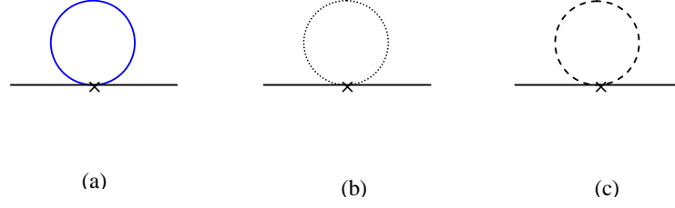
FIG. 6 One-loop diagrams giving rise to coupling renormalizations in gravity. From left to right, graviton loop, ghost loop and scalar matter loop.
