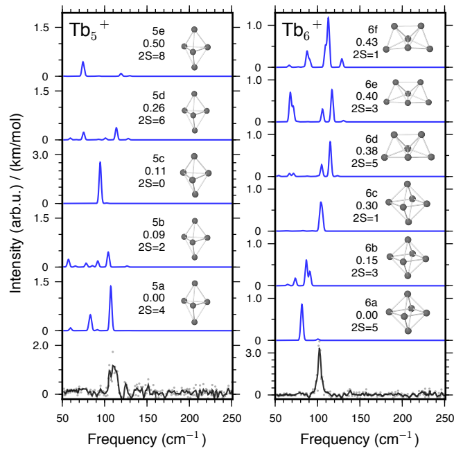
FIG. 1. Experimental far-IR spectra of \text{Tb}_5^+ and \text{Tb}_6^+ compared with the theoretically predicted spectra for a selection of low-lying structural isomers and 5d6s spin states. The experimental spectra are shown in relative cross sections \sigma \propto \nu/P(\nu) \log(I_0/I(\nu)) derived from the depletion of the Ar complexes, normalized by the photon fluence. All experimental spectra are obtained from the complexes with a single Ar atom, except for \text{Tb}_5^+ where for intensity reasons the complex has been used. To help the eye, the experimental raw data points (gray dots) are overlaid with their 5 point running average. For each isomer its energy relative to the lowest energy isomer identified (in eV) and the number of unpaired electrons 2S are given. The calculated stick spectrum is folded with a Gaussian line width function of 2 \text{cm}^{-1} full width at half maximum.
