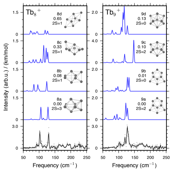
FIG. 3. Far-IR spectrum and comparison to predictions for different isomers of \text{Tb}_8^+ and \text{Tb}_9^+ .
