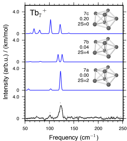
FIG. 2. Far-IR spectrum and comparison to predictions for different isomers of \text{Tb}_7^+ . Other plausible structures for \text{Tb}_7^+ , such as a capped octahedron, or bicapped pentagonal bipyramid are either significantly higher in energy, or converge to a pentagonal bipyramid under local optimization of the total energy.
