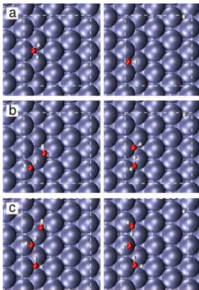
Figure 1: Structure of water clusters at the step of Pt(221) surface. Panels (a–c) show the water monomer, dimer and trimer in their intact (left) and dissociated configurations (right). The edges of the periodically replicated simulation cells used for our calculations are represented by white dashed lines.
