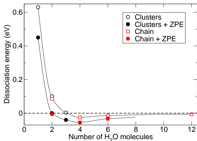
Figure 3: Dissociation energies per water molecule of clusters and periodic chains of n water molecules, with and without zero point energy (ZPE) correction. The lines are guides to the eyes and connect dissociation energy datasets with and without ZPE corrections, respectively.
