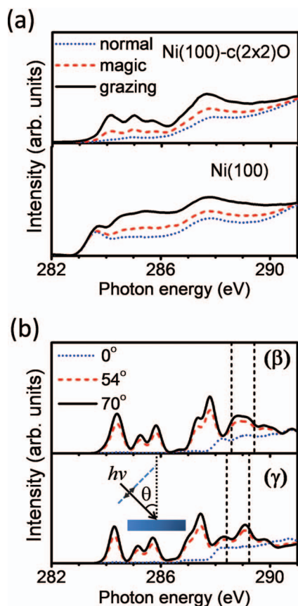
FIG. 6. (a) Experimental polarization-resolved C K-edge NEXAFS spectra for Co-OEP adsorbed on oxygen-covered ( c(2 \times 2) , top) and clean Ni(100) (bottom) referring to three different angles \theta of photon incidence, \theta = 70^\circ , 54^\circ , 0^\circ , see text. (b) Theoretical polarization-resolved C 1s core excitation spectra for the \text{Ni}_4\text{O}-(\text{Co-OEP}) cluster (top, \beta ) and the \text{Ni}_4-(\text{Co-OEP}) cluster (bottom, \gamma ), see Figs. 2(c) and 2(d). The photon incidence angles \theta , sketched in the inset, are identical to those in (a). The dashed vertical lines indicate the computed ionization potentials for the carbon species.
