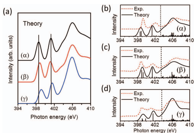
FIG. 7. (a) Theoretical N 1s core excitation spectra for ( \alpha ) the free Co-OEP molecule, ( \beta ) the \text{Ni}_4\text{O}-(\text{Co-OEP}) cluster, and ( \gamma ) the \text{Ni}_4-(\text{Co-OEP}) cluster, see text and Figs. 1 and 2. The vertical lines indicate positions of the two peaks in the free Co-OEP spectrum. (b)–(d) Comparison of the theoretical spectra ( \alpha ), ( \beta ), ( \gamma ) with corresponding experimental polarization-averaged N K-edge NEXAFS data, see text. The vertical dotted lines indicate positions of the theoretical ionization threshold in each spectrum.
