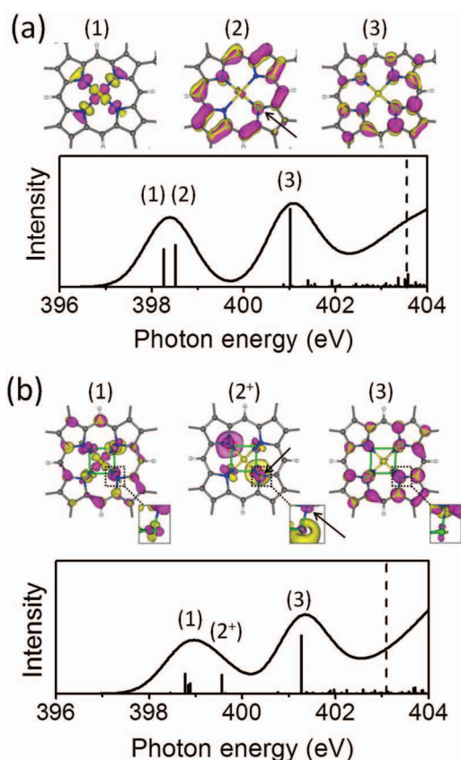
FIG. 8. Theoretical N 1s core excitation spectra for the (a) free Co-OEP molecule and (b) Ni 4 -(Co-OEP) cluster, taken from Fig. 7(a), see also text and Figs. 1 and 2. The spectra include discrete excitation energies in the double-peak region above 398 eV given by vertical lines of lengths characterizing excitation probabilities. The dashed vertical lines indicate the computed ionization potentials for the nitrogen species. The iso-surface plots above each spectrum illustrate representative final state orbitals of (1), (2), (2 + ), (3), see text. The arrows in the plots point at corresponding nitrogen excitation centers.
