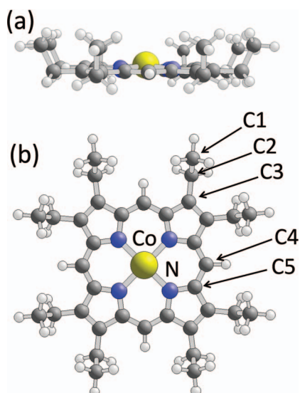
FIG. 1. Geometric structure of the free Co-OEP molecule for (a) a side view and (b) a top view. Atoms are shown by balls of different radii and labeled accordingly.
