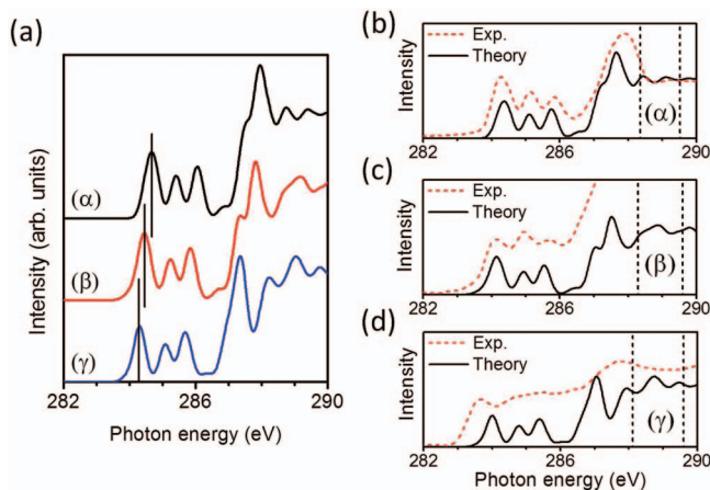
FIG. 5. (a) Theoretical polarization-averaged C 1s core excitation spectra for ( \alpha ) the free Co-OEP molecule, ( \beta ) the \text{Ni}_4\text{O}-(\text{Co-OEP}) cluster, and ( \gamma ) the \text{Ni}_4-(\text{Co-OEP}) cluster, see text and Figs. 1 and 2. The vertical lines indicate positions of the energetically lowest peak in each spectrum. (b)–(d) Comparison of the theoretical spectra ( \alpha ), ( \beta ), ( \gamma ) with corresponding experimental polarization-averaged C K-edge NEXAFS data, see text. The vertical dotted lines indicate positions of the theoretical ionization threshold in each spectrum.
