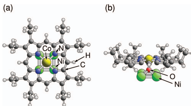
FIG. 2. Geometric structure of model clusters representing Co-OEP adsorbed at the clean and oxygen-covered Ni(100) surface, see text. (a) Top view of the \text{Ni}_4 -(Co-OEP) cluster; (b) side view of the \text{Ni}_4\text{O} -(Co-OEP) cluster. Atoms are shown by balls of different radii and labeled accordingly.
