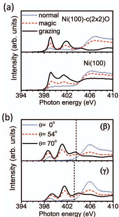
FIG. 9. (a) Experimental polarization-resolved N K-edge NEXAFS spectra for Co-OEP adsorbed on oxygen-covered (top) and clean Ni(100) (bottom) referring to three different angles \theta of photon incidence, \theta = 70^\circ, 54^\circ, 0^\circ , see text. (b) Theoretical polarization-resolved N 1s core excitation spectra for the \text{Ni}_4\text{O} -(Co-OEP) cluster (top, \beta ) and the \text{Ni}_4 -(Co-OEP) cluster (bottom, \gamma ), see Figs. 2(c) and 2(d). The photon incidence angles \theta , sketched in the inset of Fig. 6, are identical to those in (a). The dashed vertical lines indicate the computed ionization potentials for the nitrogen species.
