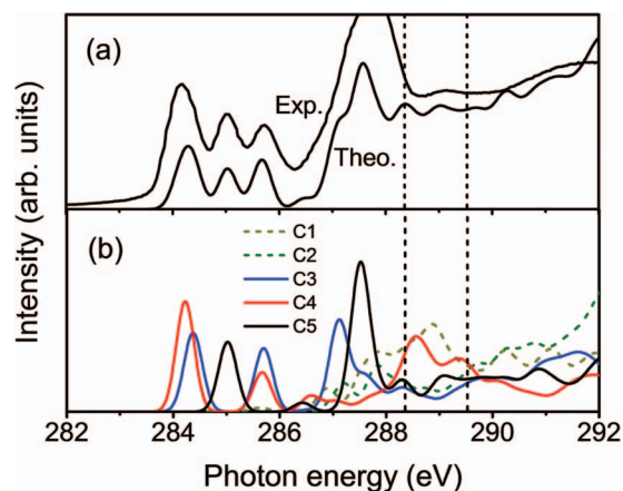
FIG. 3. (a) Theoretical C 1s core excitation spectrum of a free Co-OEP molecule (total spectrum, “Theo.”) compared with experimental C K-edge NEXAFS data (“Exp.”) for crystalline Co-OEP powder. (b) Decomposition of the total theoretical spectrum into contributions from the five non-equivalent carbon species, C1 to C5, in free Co-OEP, see Fig. 1(b). The two dashed vertical lines indicate the energy range of the computed ionization potentials for C1 to C5.
