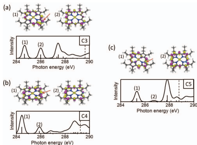
FIG. 4. Theoretical C 1s core excitation spectra of different carbon species in free Co-OEP, for (a) C3, (b) C4, and (c) C5, see Fig. 1(b). The spectra, taken from Fig. 3(b), include discrete excitation energies between 284 eV and 287 eV given by vertical lines of lengths characterizing corresponding excitation probabilities. The dashed vertical lines indicate the computed ionization potentials for the carbon species. The iso-surface plots above each spectrum illustrate representative final state orbitals (1), (2) of selected peaks labeled accordingly. The arrows in the plots point at corresponding carbon excitation centers.
