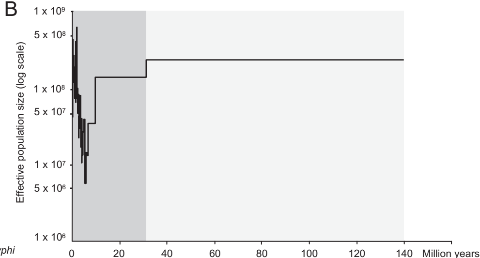
Fig. 2. Diversity and population size within E. coli .
