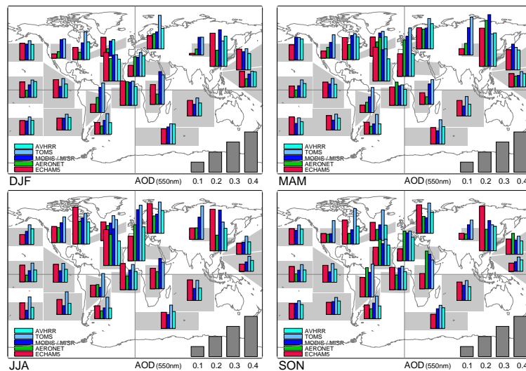
Fig. 7. Seasonal-mean aerosol optical depths ( \lambda = 550 nm) for December-January-February (DJF), March-April-May (MAM), June-July-August (JJA), and September-October-November (SON) for selected regions (gray) for the year 2000. ECHAM5-HAM (red), AERONET (green), composite of MODIS over water and MISR over land (dark blue), TOMS (light blue), and AVHRR (turquoise).
