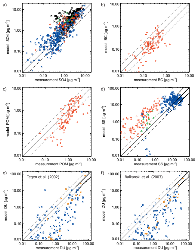
Fig. 3. Scatter plot of simulated and measured monthly mean surface aerosol mass concentrations of a) sulfate, b) black carbon, c) particulate organic matter, d) sea salt, e) dust (Tegen et al., 2002), and f) dust (Balkanski et al., 2003). Units of sulfate are \mu\text{g}(\text{SO}_4)\text{m}^{-3} and for the other compounds \mu\text{g m}^{-3} . EMEP measurements in black, IMPROVE in red, University of Miami in blue, and GAW in green. For dust, the month with the observed peak concentration is highlighted in orange. The solid line indicates the 1:1 ratio, the dashed lines the 2:1 and 1:2 ratios.
