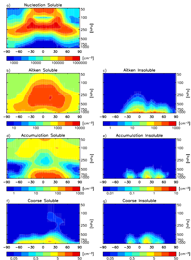
Fig. 4. Annual-mean zonal-mean number concentration for each mode [ \text{cm}^{-3} STP (1013.25 hPa, 273.15 K)].
