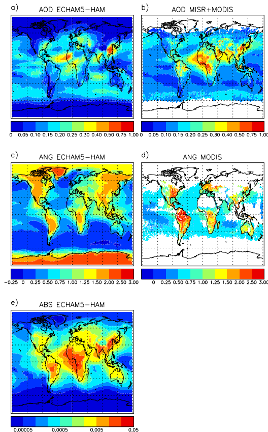
Fig. 6. Annual mean aerosol optical depth AOD simulated with ECHAM5-HAM, satellite retrieved annual (3/2000–2/2001) mean aerosol optical depth based on a composite of monthly averages of the MODIS and MISR sensors (MODIS over oceans and MISR over land), simulated 550 nm/825 nm Ångström parameter ANG of ECHAM5-HAM, satellite retrieved ANG of MODIS (ocean: 550 nm/865 nm, land: 470 nm/660 nm), simulated absorption optical depth ABS of ECHAM5-HAM. ABS and AOD refer to a mid-visible wavelength \lambda = 550 nm.
