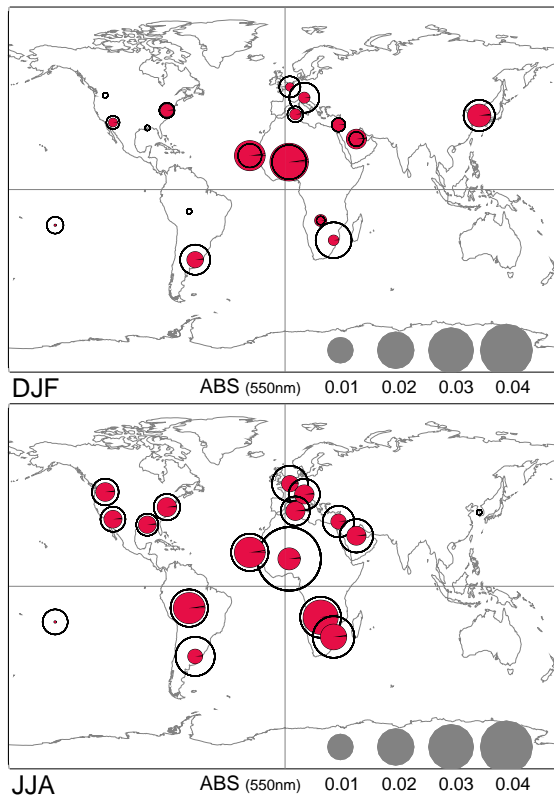
Fig. 8. Seasonal-mean absorption aerosol optical depth ABS ( \lambda = 550 nm) for December-January-February (DJF) and June-July-August (JJA) at selected AERONET sites. ECHAM5-HAM is displayed with filled red circles, AERONET with black circle lines. The absorption optical depth is proportional to the area of the circles.
