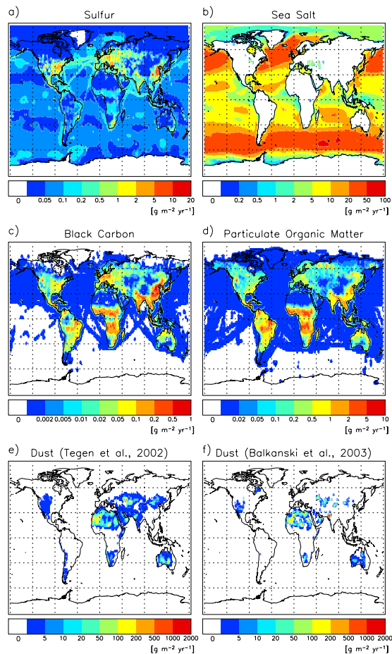
Fig. 1. Annual mean emission distribution by species. For dust emissions results of the Tegen et al. (2002) scheme and of the Balkanski et al. (2003) scheme are displayed.
