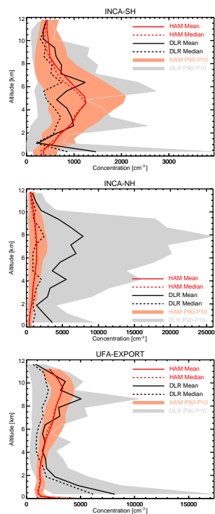
Fig. 5. Composite profiles of aerosol number-concentration [ \text{c m}^{-3} STP] from DLR aircraft measurements and ECHAM5-HAM for the INCA-SH, INCA-NH, and UFA-EXPORT measurement campaigns. ECHAM5-HAM results plotted in red, measurements in black, and the respective variability (P90-P10) in light red and gray.
