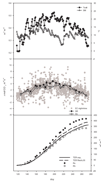
Fig. 4. Above: trend of daily average of soil temperature (–5 cm) (black dots) and soil moisture (white triangles). Middle: trend of soil respiration (black dots) and heterotrophic component of soil respiration (open dots) measured by chamber technique (error bars: \pm standard error), total ecosystem respiration by eddy covariance (grey dots) measured during night-time; Below: trend of cumulated ecosystem respiration modelled with exponential model (lower solid line), with Reichstein 2005 model (upper dashed line); cumulated soil respiration (Rs) (black dots) and heterotrophic respiration (Rh) (white dots).
