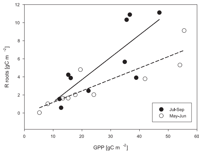
Fig. 5. Relation between root respiration (R roots) and gross primary productivity (GPP) cumulated over the periods between measurements assuming linear variation of root respiration within each period. The linear regression for the early summer (white dots, dashed line) gives a slope of 0.12 ( P < 0.01 , r^2 = 0.75 ) while for the late summer (black dots, solid line) the ratio of R roots/GPP is 0.24 ( P > 0.01 , r^2 = 0.64 ).
