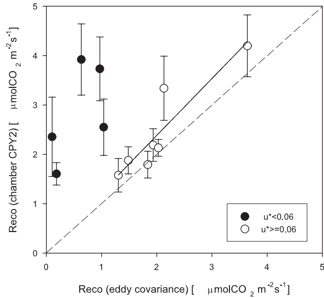
Fig. 6. comparison of eddy covariance and chamber based measurements of ecosystem respiration for conditions of friction velocity above 0.06 \text{ ms}^{-1} (white dots) and below 0.06 \text{ ms}^{-1} (black dots) . Errors bars stand for standard error of chamber \text{CO}_2 flux measurements.
