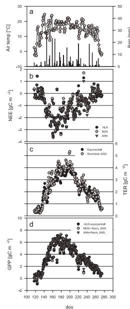
Fig. 7. (a): trend of daily average air temperature (white dots) and precipitation (black bars). (b): trend of daily NEE gapfilled with NLR, MDS and ANN methods. (c) trend of daily TER modelled with simple exponential relations and Reichstein 2005 algorithm. (d) daily GPP obtained as difference between: 1. NEE gapfilled with non linear regression method and TER modelled with simple exponential relations; 2. NEE gapfilled with MDS method and TER modelled according to Reichstein (2005); 3. NEE gapfilled with ANN method and TER modelled as in Reichstein 2005.
