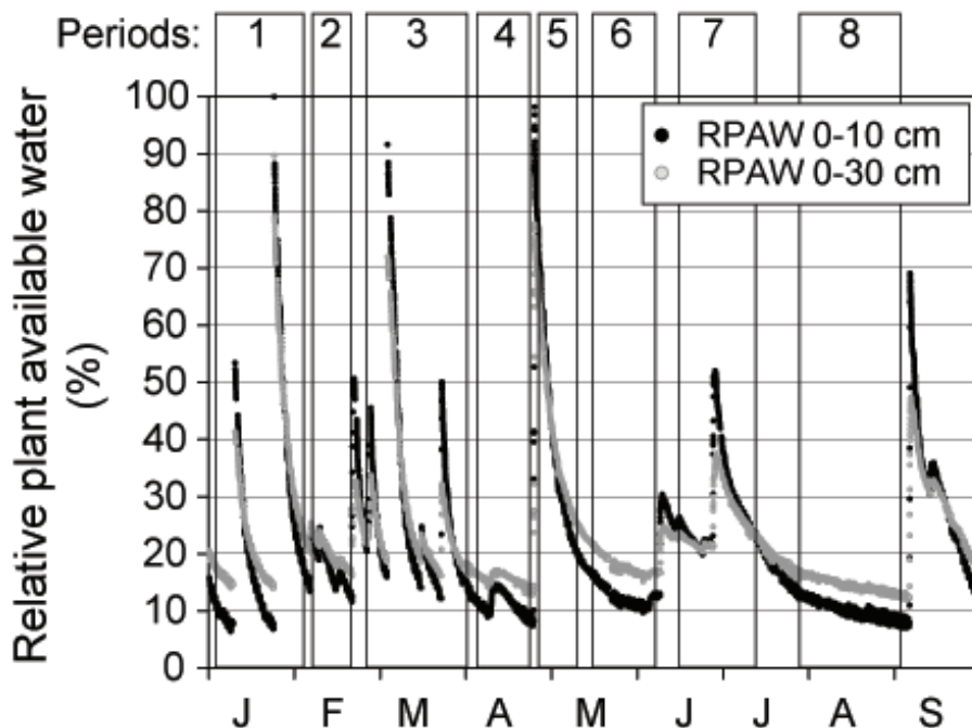
Fig. 2. Seasonal course of relative plant available water (RPAW) for the layers 0–10 cm and 0–30 cm. The periods defined in Table 1 are marked in the Figure.
