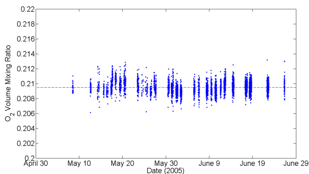
Fig. 3. O 2 volume mixing ratio. The O 2 VMR varies from 0.2061 to 0.2132. The variation comes from source brightness (solar irradiance) fluctuations during the measurements.
