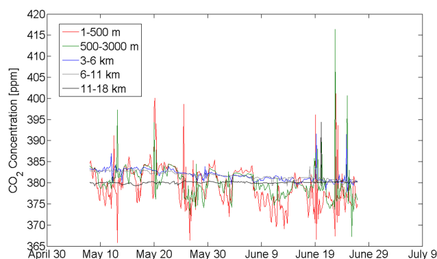
Fig. 14. Decomposition of the STILT modeled CO 2 by altitude range. The CO 2 multiple receptor signal is decomposed into the different altitude ranges of 1–500 m, 500–3000 m, 3–6 km, 6–11 km and 11–18 km. The lower altitude ranges (1–500 m and 500–3000 m), show significant influence of the biosphere in the CO 2 concentrations.
