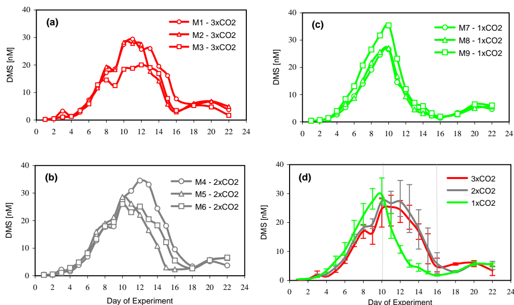
Fig. 1. DMS concentrations in nmol L -1 for the 3 enclosures of each treatment (a) 3×CO 2 (Mesocosms M1–M3) (b) 2×CO 2 (Mesocosms M4–M6) (c) 1×CO 2 (Mesocosms M7–M9) and (d) averages for all 3 treatments with range bars indicating the spread of the data. Green lines show present (1×CO 2 ), grey lines 2×CO 2 and red lines depict 3×CO 2 treatments with pCO 2 of 350 ppmv, 700 ppmv and 1050 ppmv, respectively. Horizontal dotted lines indicate the separation between the 3 phases in DMS development (see text).
