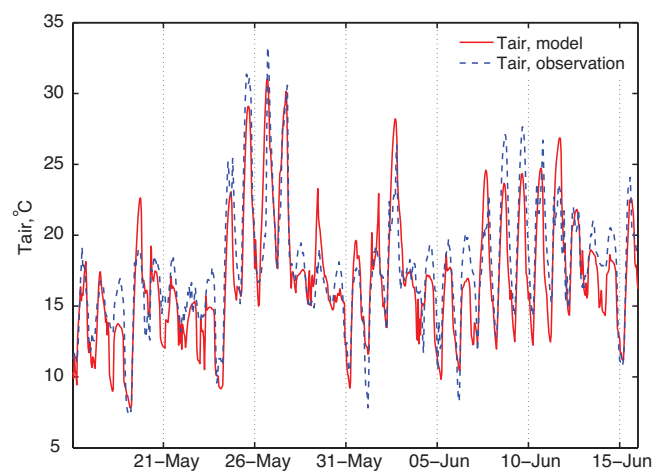
Fig. 2. Comparison of measured air temperature at 2 m with WRF simulated temperature at the meteorological station Biscarrosse Parentis. The statistics: r^2=0.77 , average bias is -0.74^\circ\text{C} , \text{RMSE}=2.14^\circ\text{C} .
