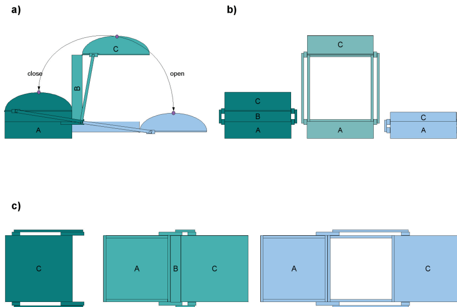
Fig. 4. Schematic overview of the BGC-FTIR Solar Tracker Dome in side (a), front (b) and top view (c). It consists of a frame of aluminum x-profile beams that are covered with aluminum plates. Its z-shaped movement is realized by two arrays of hinges and a moving lever. The middle part (Part B) is an open frame. The upper part (Part C) of the lid always faces upwards.
