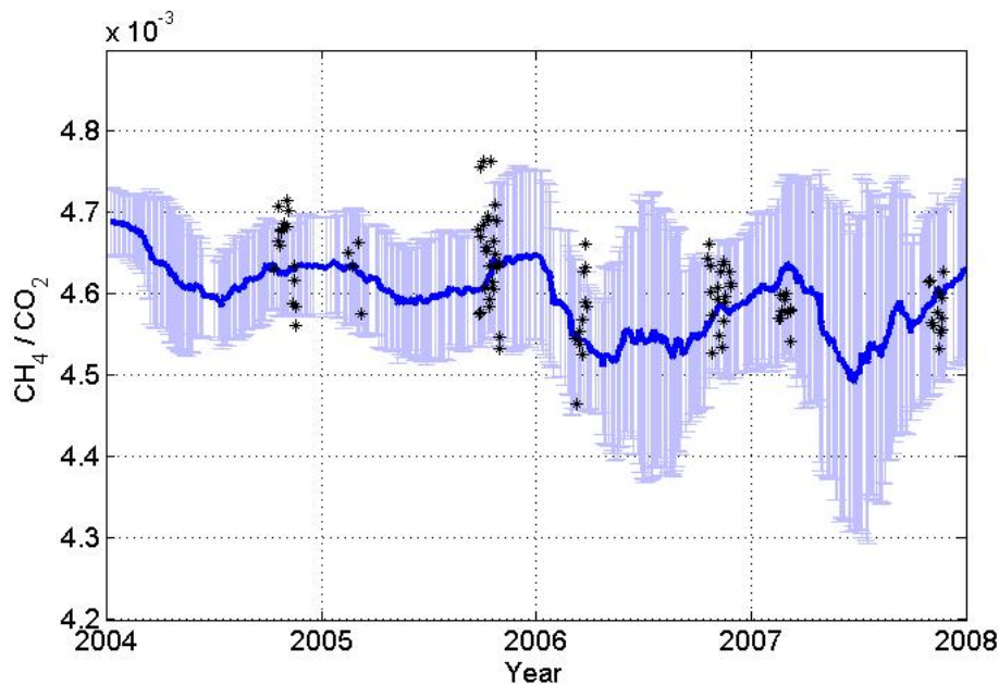
Fig. 2. \text{CH}_4/\text{CO}_2 ratios retrieved from FTIR and SCIAMACHY (IMAP-DOAS) spectra averaged over 4.0\text{--}8.0^\circ\text{N} , 54.0\text{--}57.0^\circ\text{W} . Shown is the 15-days running average over daily means from SCIAMACHY IMAP-DOAS retrieval (blue line) and the standard deviations. Due to the degradations of channel 6 of the SCIAMACHY instrument, larger standard deviations are observed in 2006 and 2007.
