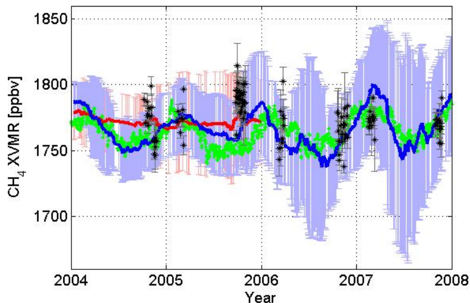
Fig. 1. Retrieved XVMR( \text{CH}_4 ) from FTIR (black stars) and SCIAMACHY spectra (IMAP-DOAS in blue, WFM-DOAS in red) averaged over 4.0\text{--}8.0^\circ\text{N} , 54.0\text{--}57.0^\circ\text{W} compared with TM5 model simulations assimilated with NOAA surface observations (green). Shown is the 15-days running average over daily means from SCIAMACHY retrievals (lines) and the standard deviations of the daily means (errorbars). The IMAP-DOAS retrieval is scaled with 1.01. Due to the degradations of channel 6 of the SCIAMACHY instrument, larger standard deviations are observed in 2006 and 2007. The FTIR observations are daily means (black stars) with standard deviations. TM3 model data for \text{CO}_2 is used to derive the XVMR( \text{CH}_4 ) in the SCIAMACHY retrievals.
