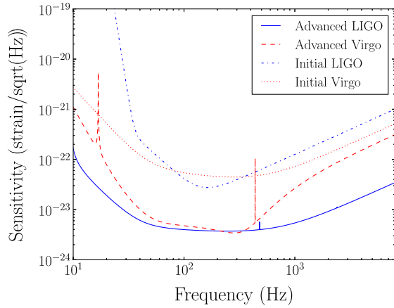
FIG. 6 (color online). The amplitude spectral density for the aLIGO zero-detuned high-power design sensitivity (blue solid curve), AdV design sensitivity (red dashed curve), initial LIGO design sensitivity (blue dot-dash curve) and initial Virgo design sensitivity (red dotted curve).
