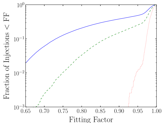
FIG. 1 (color online). The distribution of fitting factors obtained by searching for the precessing BNS systems described in Sec. II with component spins up to 0.4 (blue solid line), 0.2 (green dashed line), and 0.05 (red dotted line) using the nonspinning BNS template bank described in Sec. II and the advanced LIGO, zero-detuned, high-power PSD with a 15-Hz lower frequency cutoff.
