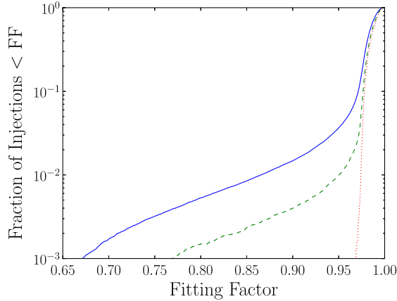
FIG. 10 (color online). The distribution of fitting factors obtained by searching for the precessing signals described in Sec. II with component spins up to 0.4 (blue solid line), 0.2 (green dashed line), and 0.05 (red dotted line) using the aligned-spin BNS template bank described in Sec. III and the advanced LIGO, zero-detuned, high-power PSD with a 15-Hz lower frequency cutoff.
