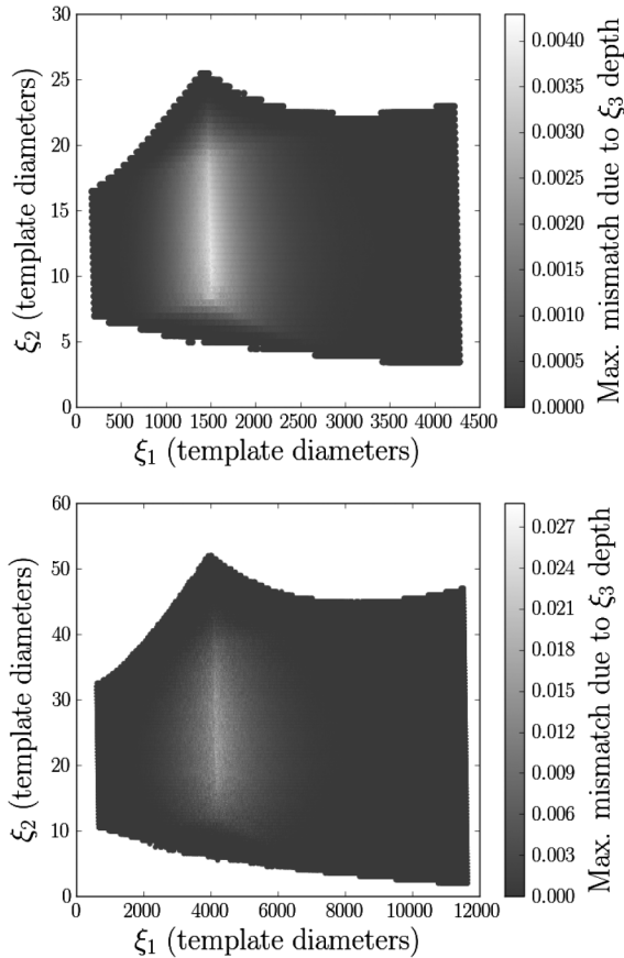
FIG. 7. The mismatch between the edge and center of the third dominant direction as a function of the first and second dominant directions when using the Virgo noise curve (top) and when using the advanced LIGO noise curve with a 10-Hz lower frequency cutoff (bottom). The \xi_i coordinates have been scaled such that one unit corresponds to the coverage diameter of a template at 0.97 mismatch. Plotted for a binary neutron star parameter space with spins restricted to 0.4.
