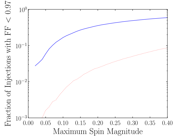
FIG. 11 (color online). The fraction of the precessing signals described in Sec. II recovered with a fitting factor less than 0.97 as a function of the maximum component spin. Shown for the nonspinning BNS template bank described in Sec. II (blue solid line), and the aligned-spin BNS template bank described in Sec. III (red dotted line). The advanced LIGO, zero-detuned, high-power PSD with a 15-Hz lower frequency cutoff was used when computing the fitting factors.
