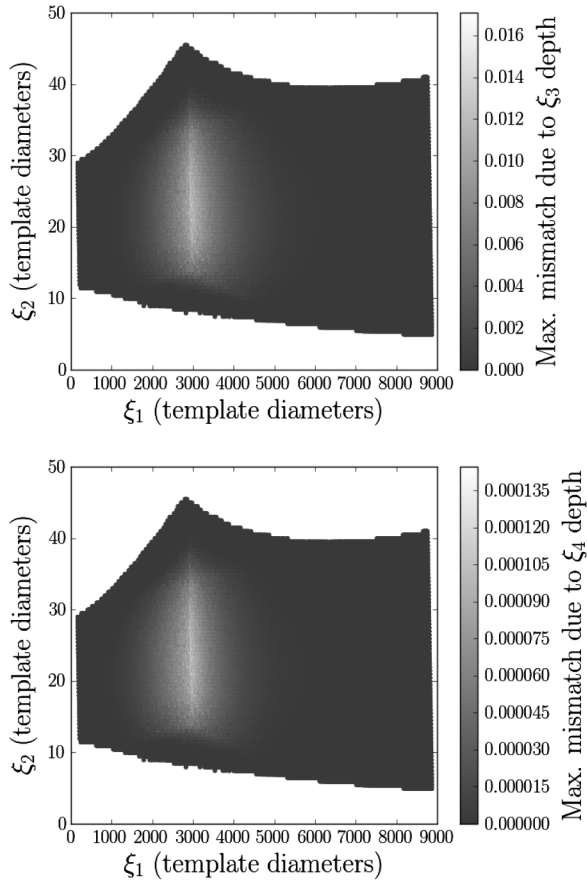
FIG. 3. The mismatch between the edge and center of the physically possible range of \xi_3 (top) and \xi_4 (bottom) values as a function of \xi_1 and \xi_2 . The \xi_i coordinates have been scaled such that one unit corresponds to the coverage diameter of a template at 0.97 mismatch. Plotted for a binary neutron star parameter space with spins restricted to 0.4 using the zero-detuned, high-power advanced LIGO sensitivity curve with a 15-Hz lower frequency cutoff.
