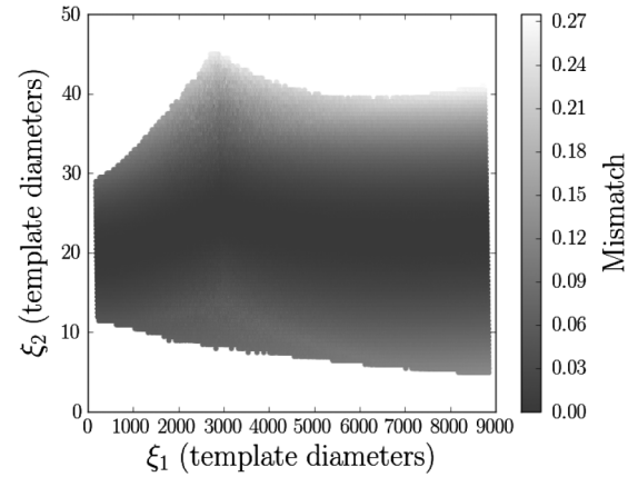
FIG. 9. The mismatch between unphysical \eta and aligned-spin BNS templates as a function of the first and second dominant directions. In making this plot we assume that \xi_3 has no depth in the aligned spin case by taking the central value where \xi_3 has a range of values. This plot was generated with spins restricted to 0.4 using the zero-detuned, high-power advanced LIGO sensitivity curve with a 15-Hz lower frequency cutoff.
