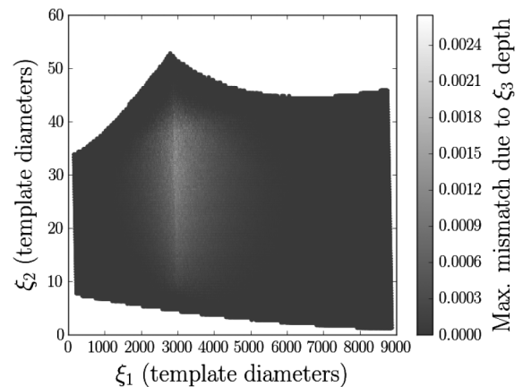
FIG. 8. The mismatch between the edge and center of the third dominant direction as a function of the first and second dominant directions using waveforms incorporating the subdominant spin corrections to the orbital phase. The \xi_i coordinates have been scaled such that one unit corresponds to the coverage diameter of a template at 0.97 mismatch. Plotted for a binary neutron star parameter space with spins restricted to 0.4 using the zero-detuned, high-power aLIGO sensitivity curve with a 15-Hz lower frequency cutoff.
