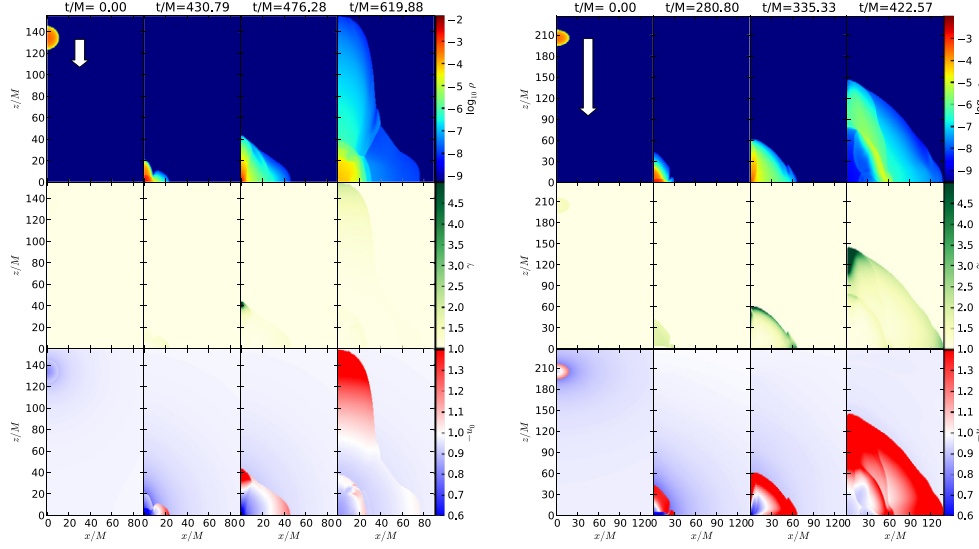
Figure 1. Representative snapshots of the rest-mass density, \rho , in units where c = 1 = M_{\odot} (top row), of the Lorentz factor, \gamma (middle row), and of the local fluid energy, -u_0 (bottom row), for subcritical models with an initial small boost v_b/c = 0.3 (left panel) or a large one v_b/c = 0.8 (right panel). Note that the post-collision flow is essentially jet-like for the low-boost case (left panel), while essentially spherical for the high-boost case (right panel); in this latter case, most of the matter is unbound.
