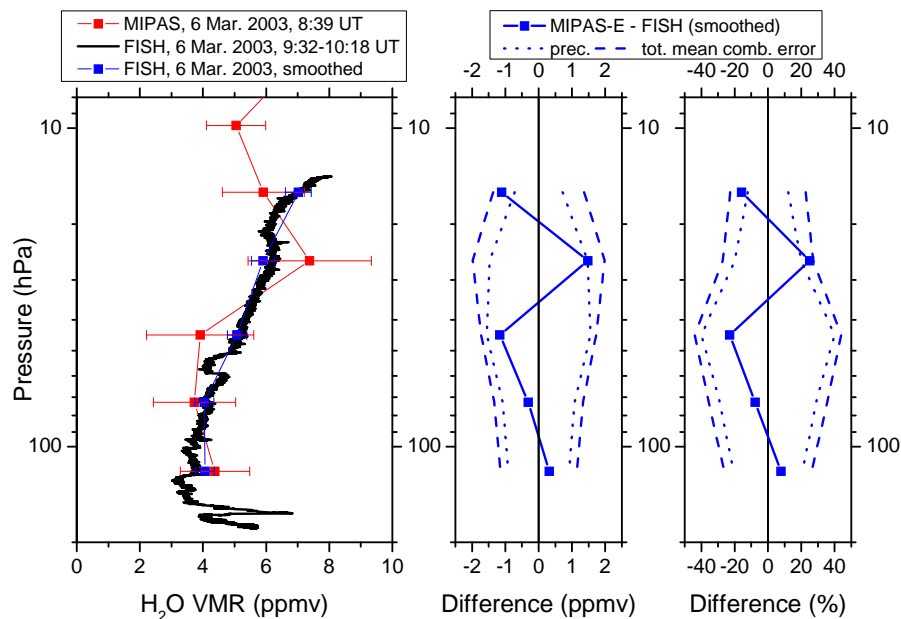
Fig. 5. Direct comparison of H 2 O profiles measured by MIPAS-E and the balloon-borne in-situ instrument FISH on 6 March 2003 at Kiruna (~68°N) along with absolute and relative differences and combined errors. The in-situ FISH profile was smoothed with the averaging kernel of MIPAS-E to make the vertical resolution of both instruments comparable. Annotation as per Fig. 4.
