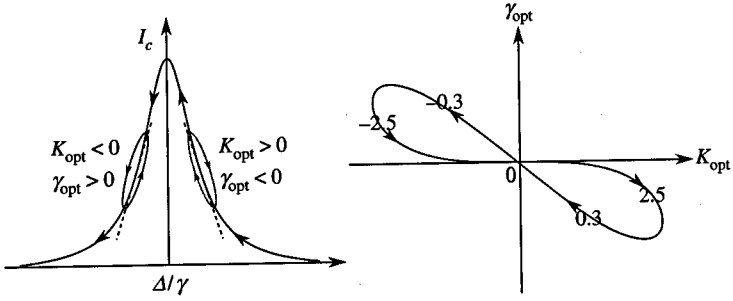
Figure 15.13 The optical power as a function of cavity detuning \Delta (left) and a double optical spring (right), of which the total rigidity is sum of individual values K_{tot}(\Omega) = K_1(\Omega) + K_2(\Omega) .
