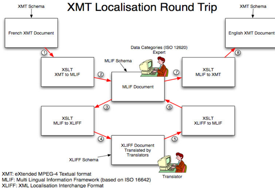
Figure 17: XMT-O Localization Roundtrip.
