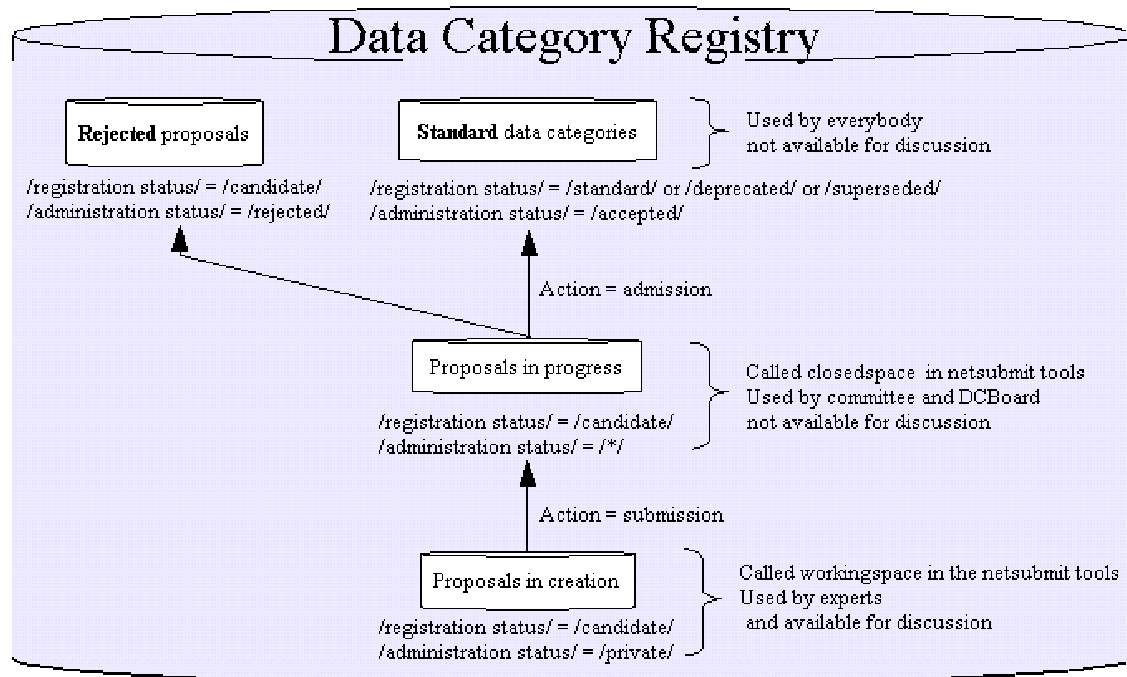
Figure 3: Behaviour of a Data Category Registry.
