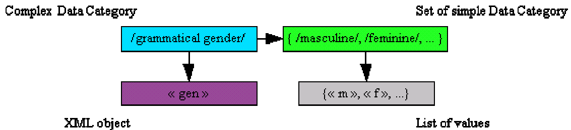
Figure 2: Example with the complex Data Category /grammatical gender/.
