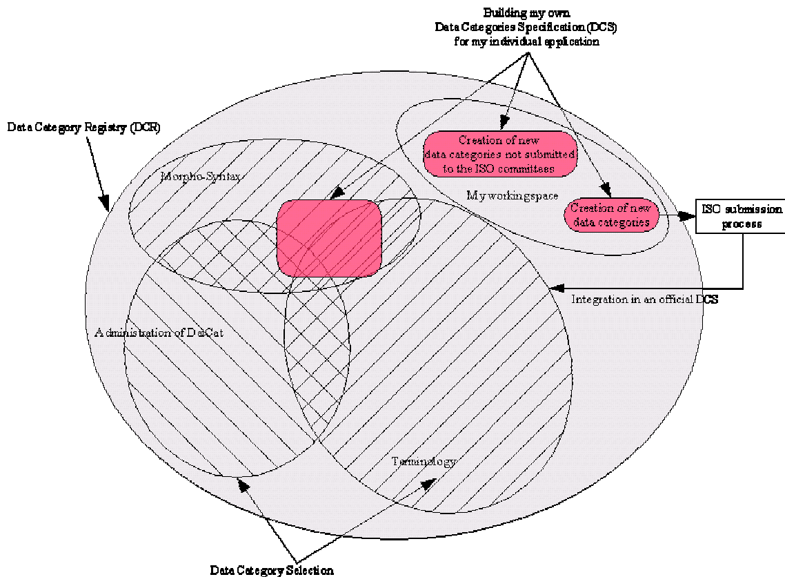
Figure 4: Data Categories (DatCat), Data Categories Selection (DCS) and Data Category Registry (DCR).
