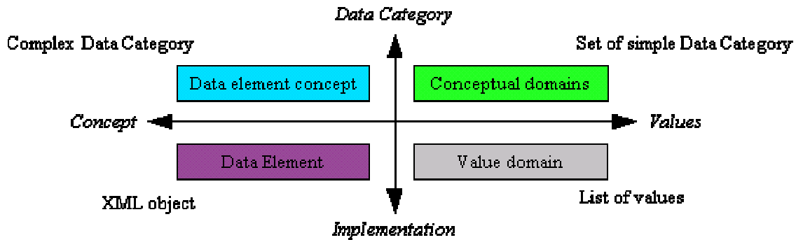
Figure 1: Data Categories from ISO 11179.
