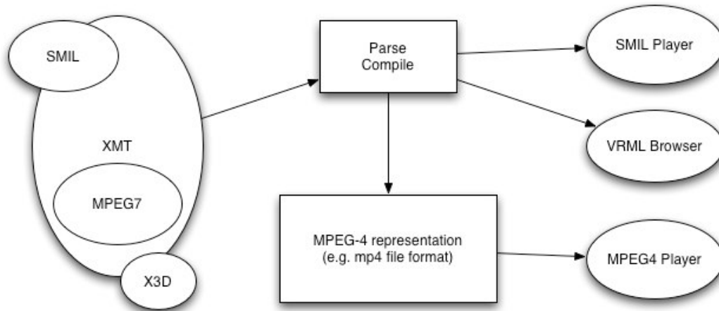
Figure 14: Interoperability of XMT with other standards.
