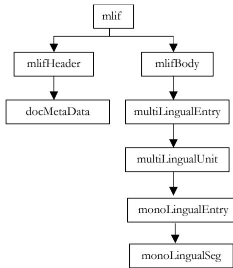
Figure 7: Hierarchical representation of MLIF.
