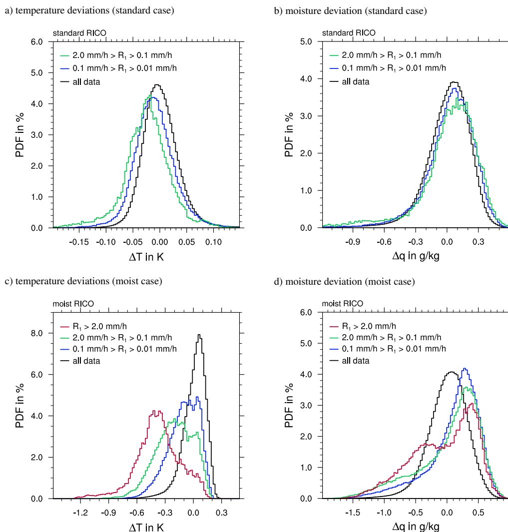
Fig. 9. Histograms of the sub-cloud temperature and moisture anomalies, for all data and conditioned on precipitation rate. The precipitation rate R_1 is averaged over 15 min in time, and precipitation rate and anomalies are averaged spatially over 1 \text{ km} \times 1 \text{ km} . Simulations R01 and M01-big sampled over 20 h to 40 h. Note that in contrast to Fig. 8 all conditional PDFs are normalized to 1.
