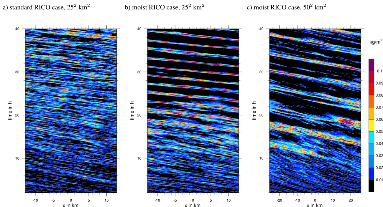
Fig. 4. Hovmöller diagrams of y -averaged cloud liquid water path for three different simulations of the RICO trade wind cumulus case. The standard GCSS RICO case on (a) a 25 \text{ km} \times 25 \text{ km} domain and (b) the moist case on the same domain and (c) the moist case on a 50 \text{ km} \times 50 \text{ km} domain.
