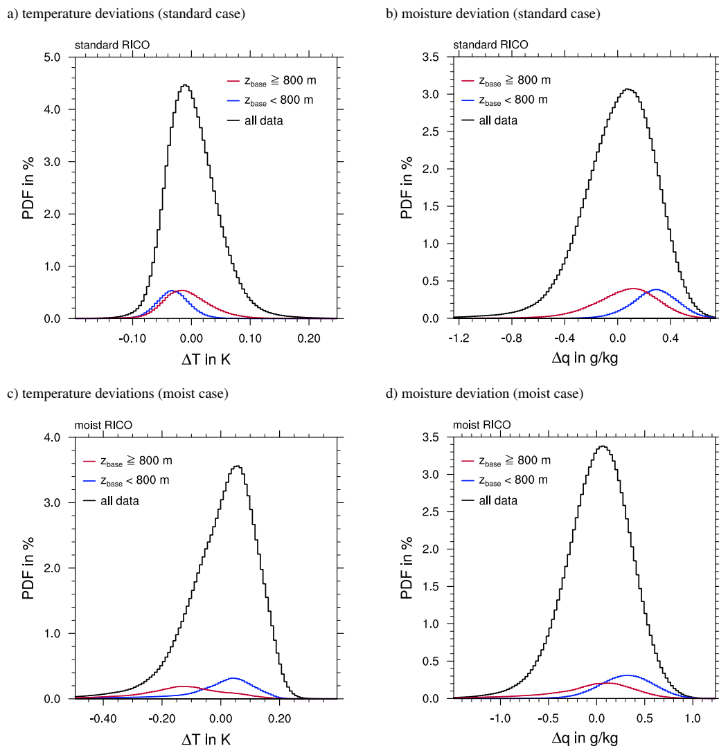
Fig. 8. Histograms of the sub-cloud temperature and moisture anomalies, for all data and sub-sampled for cloudy columns with cloud base below and above 800 m, i.e., the colored lines indicate that part of the PDF which is cloudy with a certain cloud base. Simulation R01 and M01-big sampled over 20 h to 40 h.
