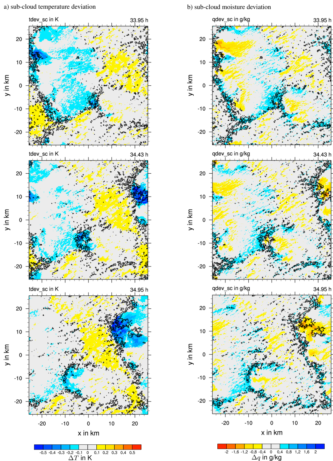
Fig. 7. Temperature (left) and moisture (right) deviation in the sub-cloud layer at different simulation times corresponding to Fig. 1. Isolines show the liquid water path with contour lines at 0.01 \text{ g m}^{-2} and 1.0 \text{ g m}^{-2} (black).
