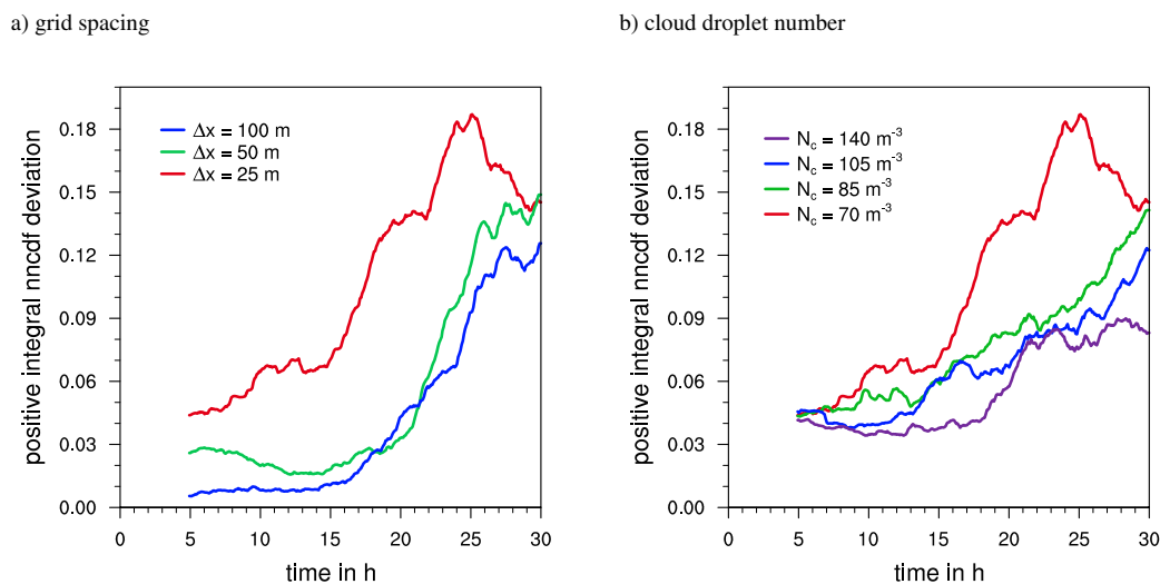
Fig. 10. Time series of the positive integral deviation of the nearest neighbor cumulative distribution (higher values indicate stronger clustering). Shown are the simulations M01, M12 and M13 (left) and M01 together with M14–M16 (right).
