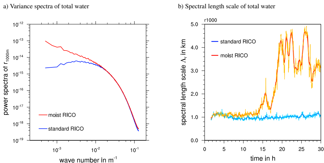
Fig. 5. Power spectra (left) and time series of the spectral length scale \Lambda_r (right) of the total water mixing ratio at 1000 m height for the standard and moist RICO case on the 25 \text{ km} \times 25 \text{ km} domain (in the time series plot the red and dark blue lines represent 30 min running averages, orange and light blue lines show the corresponding 1 min data).
