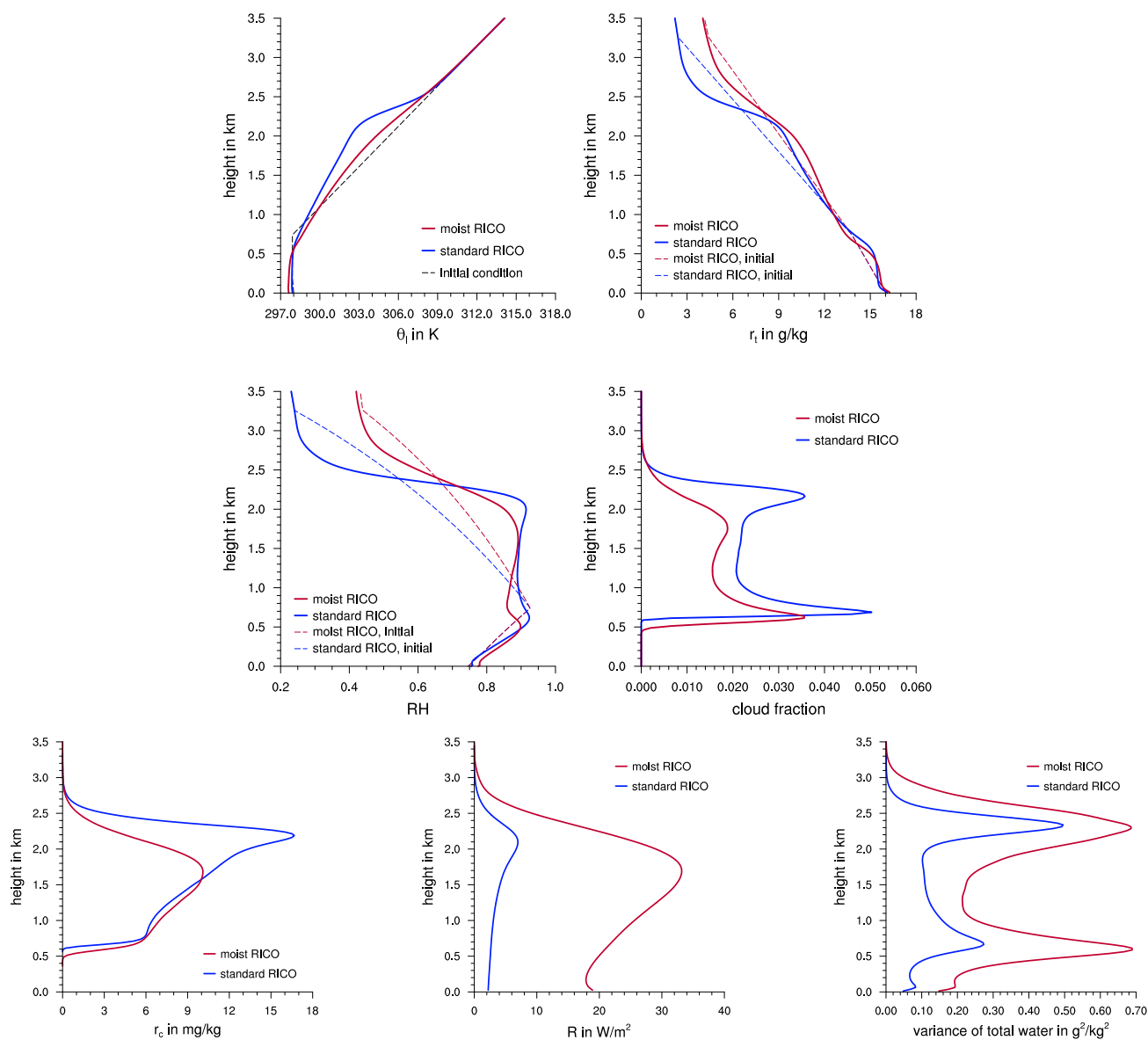
Fig. 3. Mean profiles of the standard GCSS RICO case (blue) and the moist RICO case (red) with the corresponding initial conditions (dashed) on the 25 km \times 25 km domain. Profiles are averages over the entire domain from 24 h to 30 h of the simulation. Shown in upper panels from left to right are liquid water potential temperature and total water mixing ratio, and in the 2nd row relative humidity and cloud fraction. On lower panels from left to right are cloud liquid water mixing ratio, rain water flux and the variance of the total water mixing ratio. The rain water flux profile is conditionally averaged over the raining areas.
