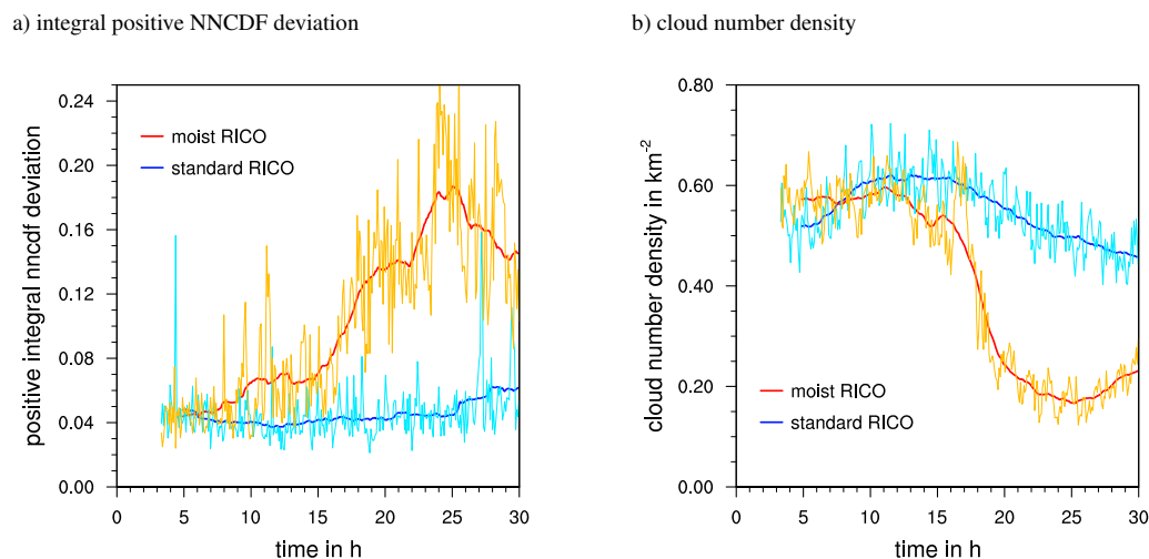
Fig. 6. Time series of the positive integral deviation of the nearest neighbor cumulative distribution (left, higher values indicate stronger clustering) and cloud number density (right) (in the time series plot the red and dark blue lines represent 120 min running averages, orange and light blue lines show the corresponding 1 min data).
