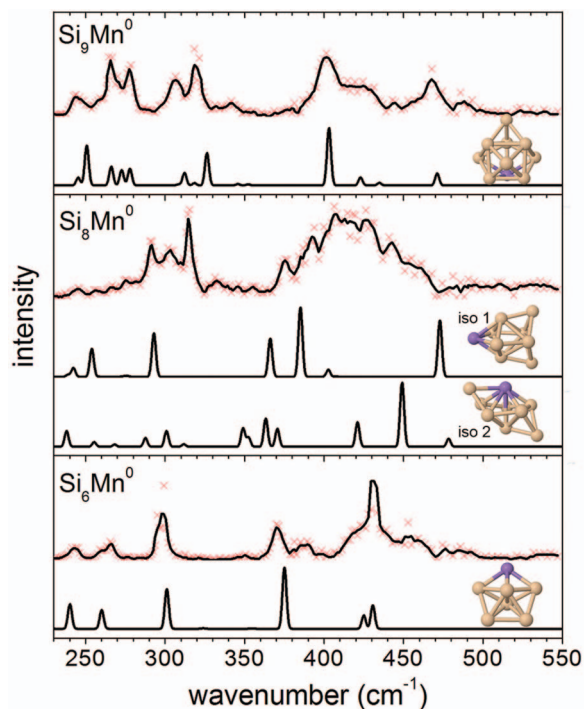
FIG. 3. IR-MPD spectra (upper traces) of \text{Si}_n\text{Mn} \cdot \text{Xe} complexes ( n = 6, 8, 9 ) and the corresponding calculated vibrational spectra of the xenon complexes of the lowest-energy isomers (lower traces). For \text{Si}_8\text{Mn} , the second lowest-lying isomer is also presented. The geometries are shown as insets next to their corresponding computed vibrational spectra. The experimental data points (red crosses) are overlaid with a three-point running average. The computed infrared spectra are calculated at the B3P86/6-311+G(d) level.
