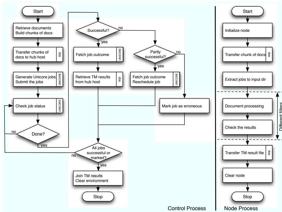
Figure 2: The TMGrid workflow. The actual processing stage on one Grid cluster node can be substituted by modules as appropriate. Limitations in UNICORE data staging force part of the workflow to be handled by the wrapper shell script.
