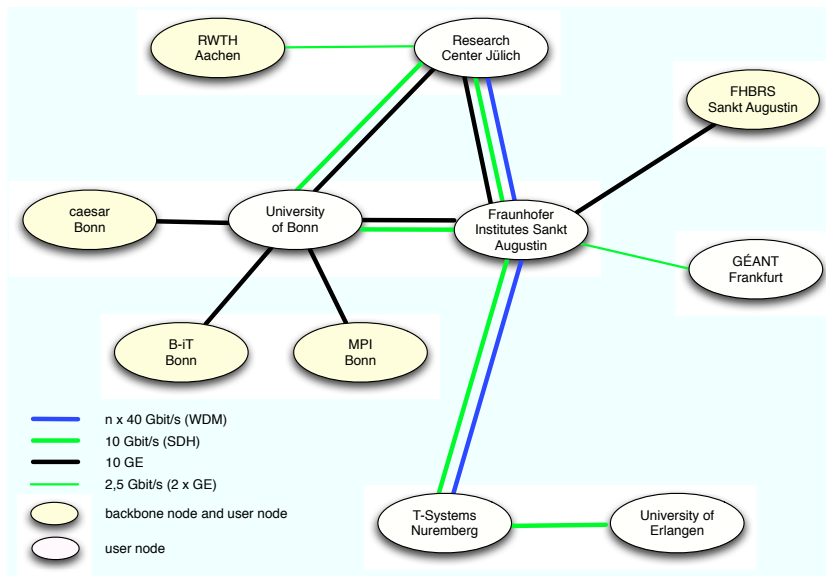
Figure 1: VIOLA (Vertically Integrated Optical testbed for Large Applications) Topology
