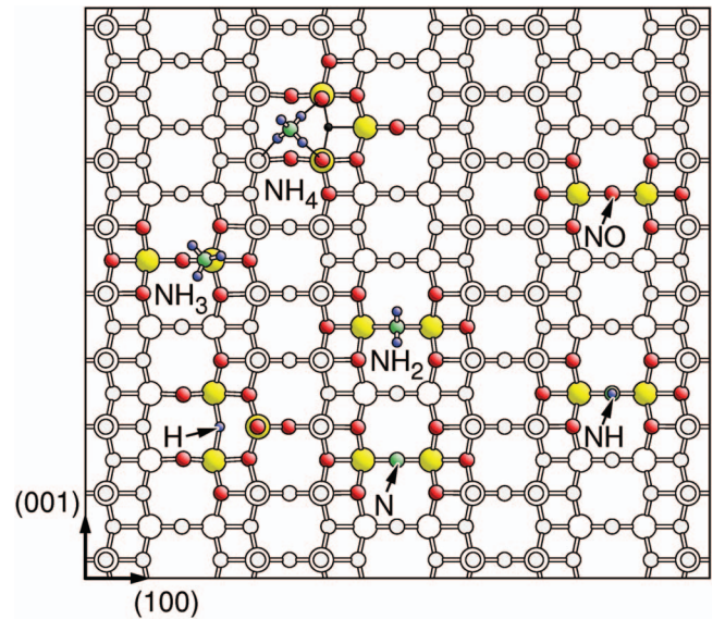
FIG. 5. Energetically most preferred equilibrium structures of H, N, NO, and \text{NH}_x ( x = 1, \dots, 4 ) at the reduced \text{V}_2\text{O}_5(010) surface, see text. Vanadium atoms are shown by large yellow balls, oxygen and nitrogen centers by smaller red and green balls, respectively, and hydrogen by very small blue balls. Surface atoms that are included in the optimization (in addition to the adsorbate) are shown as painted balls. Oxygen vacancy centers are indicated by small black dots.
