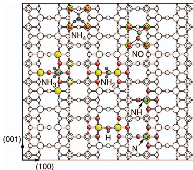
FIG. 3. Energetically most preferred equilibrium structures of H, N, NO, and \text{NH}_x ( x = 1, \dots, 4 ) at the perfect \text{V}_2\text{O}_5(010) surface, see text. Vanadium atoms are shown by large yellow balls, oxygen and nitrogen centers by smaller red and green balls, respectively, and hydrogen by very small blue balls. Surface atoms that are included in the optimization (in addition to the adsorbate) are shown as painted balls.
