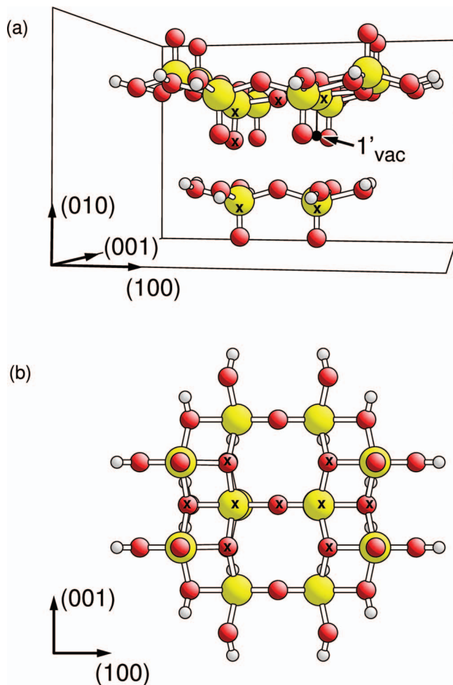
FIG. 6. Sub-surface oxygen O(1') vacancy cluster V_{12}O_{39}H_{20}^* , in (a) perspective and (b) top view. Vanadium centers are shown by large yellow balls, oxygen centers by smaller red balls, and very small gray balls refer to hydrogen centers. The position of the missing oxygen atom is indicated by a small black dot. Atoms considered in the geometry optimization are labeled by a cross.
