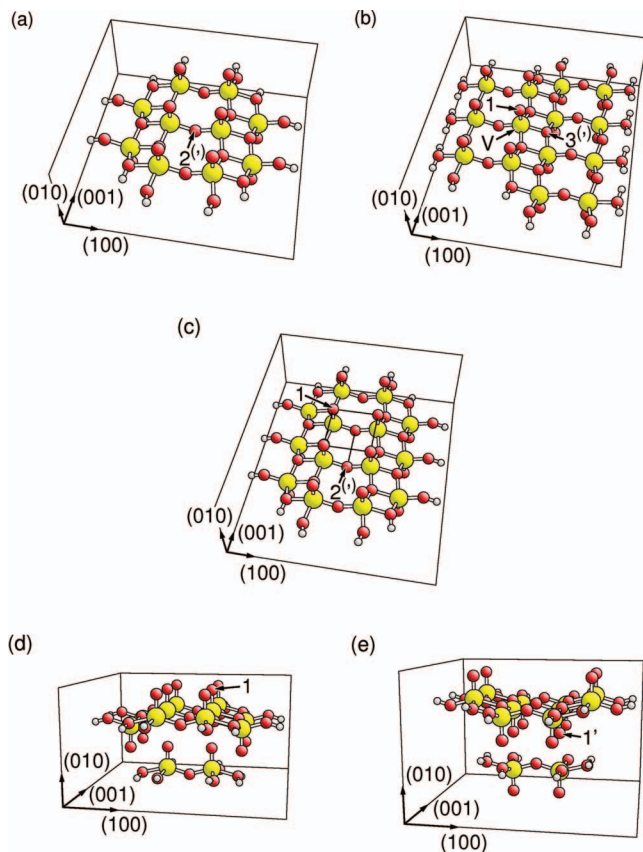
FIG. 2. Cluster models used to model different sections of the perfect and reduced V_2O_5(010) surface: (a) V_{10}O_{31}H_{12} , (b) V_{14}O_{46}H_{22} , (c) V_{14}O_{42}H_{14} , (d) V_{12}O_{40}H_{20} , and (e) V_{12}O_{40}H_{20}^* , see text. Vanadium atoms are shown by large yellow, oxygen by smaller red, and saturating hydrogen by very small gray balls. Corresponding oxygen sites are labeled accordingly.
