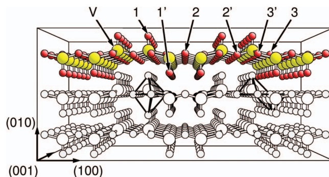
FIG. 1. Crystal structure of orthorhombic \text{V}_2\text{O}_5 for a view along the (001) direction (perpendicular to the (010) direction). The topmost physical (010) layer is emphasized by shading. Vanadium atoms are shown by large yellow and oxygen by smaller red balls. Neighboring atom centers are connected by sticks to visualize structural properties. The non-equivalent oxygen centers, \text{O}(1^{(l)}-3^{(l)}) of the crystal surface are labeled accordingly, see text. In the second physical layer, the shapes of octahedral \text{VO}_6 (left) and bipyramidal \text{V}_2\text{O}_8 (right) crystal building units are outlined.
