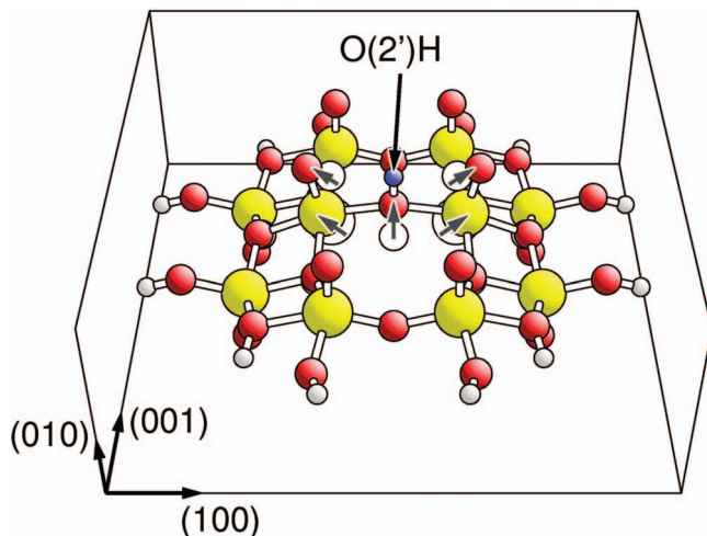
FIG. 4. Equilibrium geometry of hydrogen adsorbed at the O(2') site of the perfect V_2O_5(010) surface. Vanadium centers are shown by large yellow balls, oxygen centers by smaller red balls, adsorbed hydrogen by very small blue balls and saturating hydrogen by small bright gray balls. Surface atom positions before adsorption are indicated by white balls.
