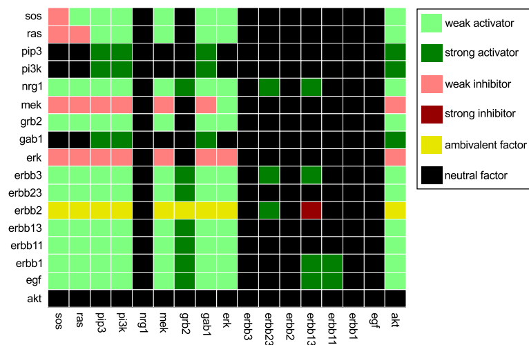
Figure 3 Dependency matrix of the EGF/NRG1 example model given in Figure 2A. The color of row i , column j shows the influence of species i on species j .
