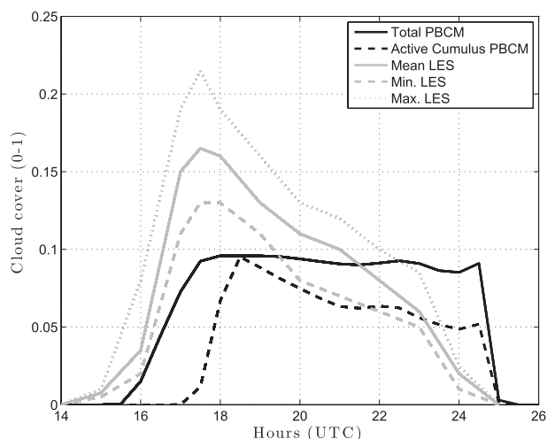
FIG. 10. PBCM total (continuous black line) and active cloud cover (dashed black line) compared to the mean (continuous gray line), minimum (dashed gray line), and maximum (dotted gray lines) LES outputs of Brown et al. (2002).
