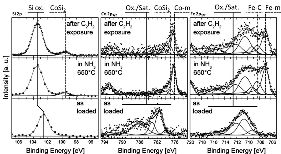
Fig. 9 (From left to right) APXP spectra of the Si 2p, Co 2p 3/2 and Fe 2p 3/2 regions showing the evolution of the surface (Fe, Co; E_{kin}(e^-) = 150 eV) and near surface (Si; E_{kin}(e^-) = 1000 eV) chemistry under low pressure CVD. Reproduced with permission from ref. 126.
