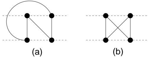
Fig. 3. (a) A planar bipartite graph that is (b) not 2-level planar
