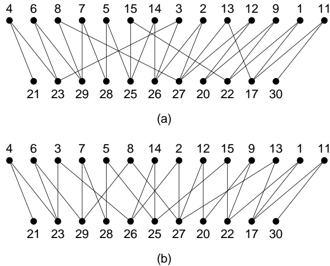
Fig. 2. A graph (a) drawn using k -planarization and (b) drawn with the minimal number of crossings computed by the algorithm in [JM96]
