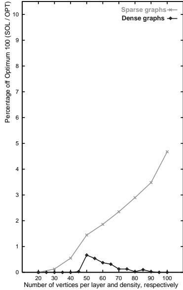
Fig. 7. Results for 100 instances
