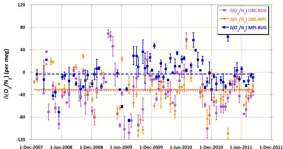
Fig. 4. Differences of the \delta(\text{O}_2/\text{N}_2) values measured by each set of two laboratories. Also indicated are the average differences. These are: -33 per meg for UBE-RUG, -31 per meg for UBE-MPI and -3 per meg for MPI-RUG. The error bars represent the quadratically added standard errors of the measurements of the two laboratories.
