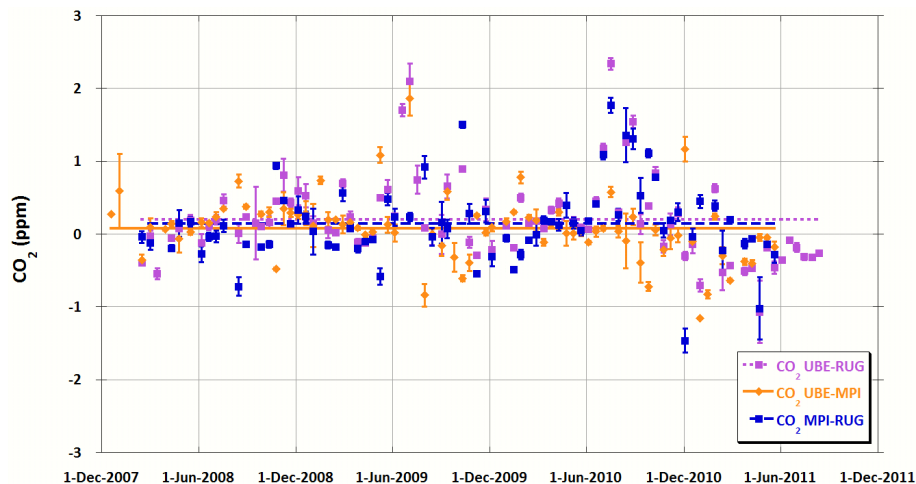
Fig. 2. Differences of the CO 2 concentration measured by each set of two laboratories. Also indicated are the average differences. These are: 0.20 ppm for UBE-RUG, 0.08 ppm for UBE-MPI and 0.14 ppm for MPI-RUG. The error bars represent the quadratically added standard errors of the measurements of the two laboratories.
