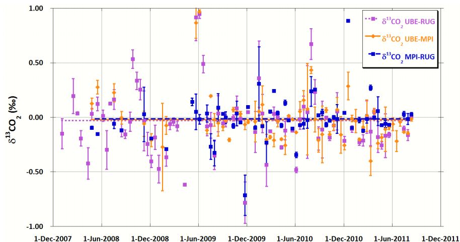
Fig. 6. Differences of the \delta^{13}\text{CO}_2 values measured by each set of two laboratories. Also indicated are the average differences. These are: -0.03\text{‰} for UBE-RUG, -0.02\text{‰} for UBE-MPI and -0.02\text{‰} for MPI-RUG. The error bars represent the quadratically added standard errors of the measurements of the two laboratories.
