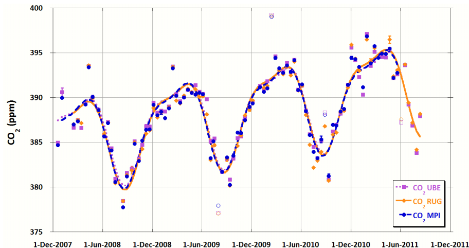
Fig. 1. CO 2 concentration at Jungfraujoch, Switzerland from flask samples measured by three laboratories: University of Bern (UBE) (pink squares), University of Groningen (RUG) (orange diamonds) and Max Planck Institute in Jena (MPI) (blue circles). The values are the averages of 1, 2 or 3 flasks. The fits through the data are linear trends and double harmonic seasonal. Open symbols represent those values that are outliers to the fit of the individual data set. The error bars represent the standard error of the average value of 2 or 3 flasks. For single flask measurements error bars are not shown.
