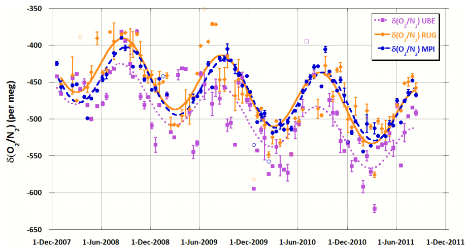
Fig. 3. \delta(\text{O}_2/\text{N}_2) observations from Jungfraujoch, Switzerland from flask samples measured by three laboratories: UBE (pink squares), RUG (orange diamonds) and MPI (blue circles). The values are the averages of 1, 2 or 3 flasks. The fits through the data are linear trends and single harmonic seasonal components. Open symbols represent those values that are outliers to the fit of the individual data set. The error bars represent the standard error of the average value of 2 or 3 flasks. For single flask measurements error bars are not shown.
