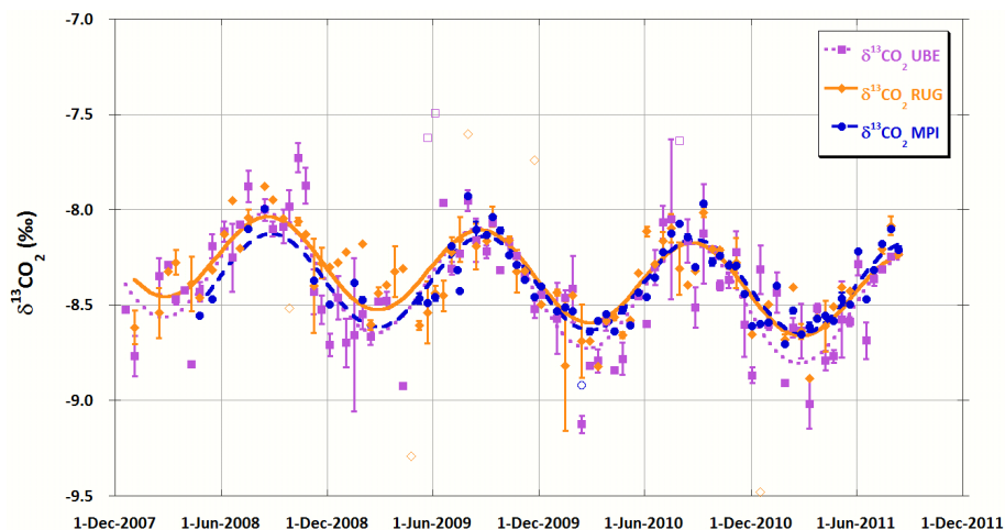
Fig. 5. \delta^{13}\text{CO}_2 observations from Jungfraujoch, Switzerland from flask samples measured by three laboratories: UBE (pink squares), RUG (orange diamonds) and MPI (blue circles). The values are the averages of 1, 2 or 3 flasks. The fits through the data are linear trend and single harmonic seasonal components. Open symbols represent those values that are outliers to the fit of the individual data set. The error bars represent the standard error of the average value of 2 or 3 flasks. For single flask measurements error bars are not shown.
