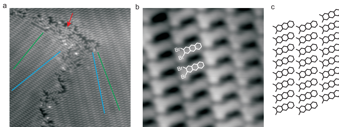
Figure 5.16: a , 38 \times 38 \text{ nm}^2 STM overview of tdBA on Au(111) without a heating step. The blue and green lines denote the molecule-island and crystal orientation, respectively. The red arrow indicates a domain boundary with a reduced order. b , 10 \times 10 \text{ nm}^2 STM image. Chemical structures indicate the adsorption geometry of the molecules. c , Schemed arrangement of the tdBA islands.
