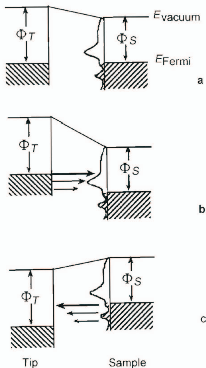
Figure 2.2: Energy levels contributing to the tunneling current. \Phi_T and \Phi_S are the work functions of the tip and the sample, respectively. a , Zero bias: no current. b , Positive sample bias: Occupied tip states tunnel into unoccupied sample states. c , Negative sample bias: Occupied sample states tunnel into unoccupied tip states. From [37]. This material is reproduced with permission of John Wiley & Sons, Inc.
