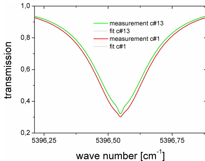
Fig. 9. A H 2 O line as observed in a calibration measurement. The narrow dip appended to the line center is due to absorption at low pressure, while the strong underlying absorption is generated in the lab air path. The superimposed dashed lines are synthetic spectra generated with LINEFIT.
