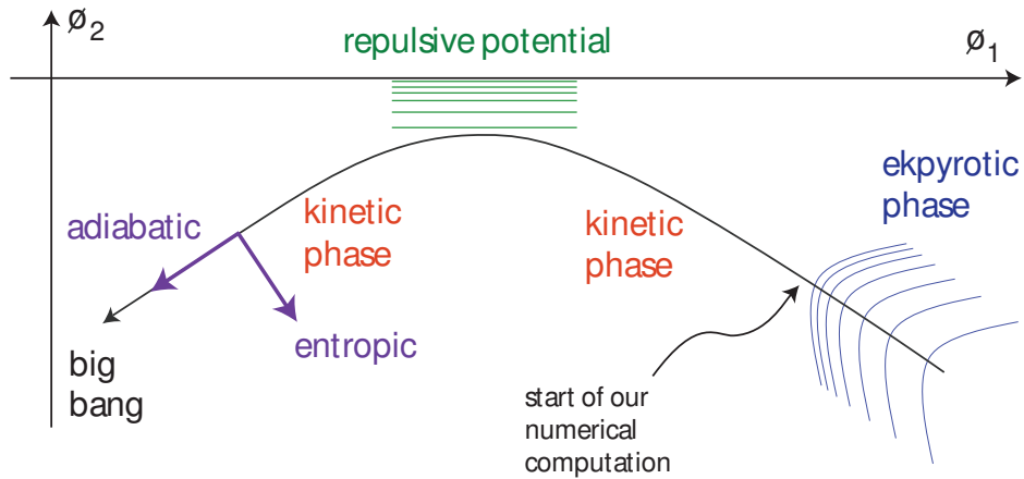
FIG. 1: In the models that we study, the evolution starts out with an ekpyrotic contracting phase to the right of the figure. During this phase, nearly scale-invariant entropy perturbations, which are perturbations transverse to the background trajectory, are amplified and evolve into a highly squeezed quantum state. Such a squeezed quantum state is approximately classical in the sense that it can equivalently be described as a statistical mixture of classical perturbations. After the ekpyrotic phase, the trajectory in scalar field space enters the kinetic phase and bends - this bending causes the conversion of entropy into curvature perturbations, with the latter inheriting both their spectrum and their near-classicality from the entropy perturbations. Moreover, the interactions of entropy and curvature modes during the bending phase cause decoherence to occur, such that the resulting curvature perturbations can be assigned definite classical probabilities for their amplitude. In this way, the ekpyrotic phase produces an ensemble of nearly scale-invariant classical density perturbations in the approach to the bounce.
