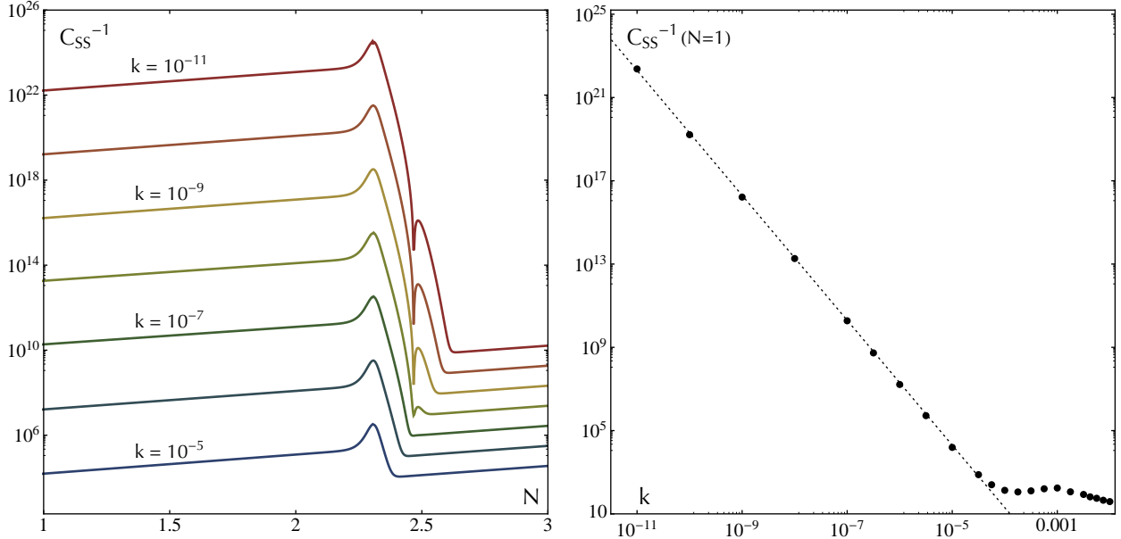
FIG. 3: The figure shows the amplification of the curvature perturbations (\Delta v)^2 = 1/C_{SS} as a function of time (left panel) and at the reference time N = 1 (right panel) for various wavenumbers k . Noting the logarithmic scale on the vertical axis, it is evident that long-wavelength modes become highly amplified during the conversion process. In particular, at fixed time one finds (\Delta v)^2 \propto k^{-3} . During the kinetic phase, this amplification is reduced somewhat, but will remain large if the bounce occurs within not too large a number of e-folds after conversion.
