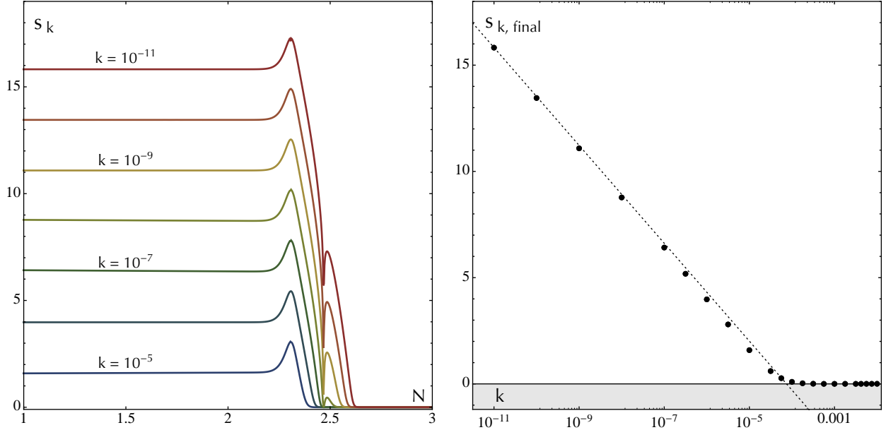
FIG. 2: These figures show the entanglement entropy s_k as a function of time for various wavenumbers k . Time runs from the right to the left, and is given in units of scale-factor time N \propto \ln(a) . Left panel: the perfect quantum coherence at the end of the ekpyrotic phase is rapidly destroyed during the conversion process, and reaches a constant value in the approach to the bounce. Right panel: for small-wavelength modes, the final amount of decoherence s_{k,final} can be seen to be inversely proportional to k – the dashed line corresponds to the fitting formula ((III.13)).
