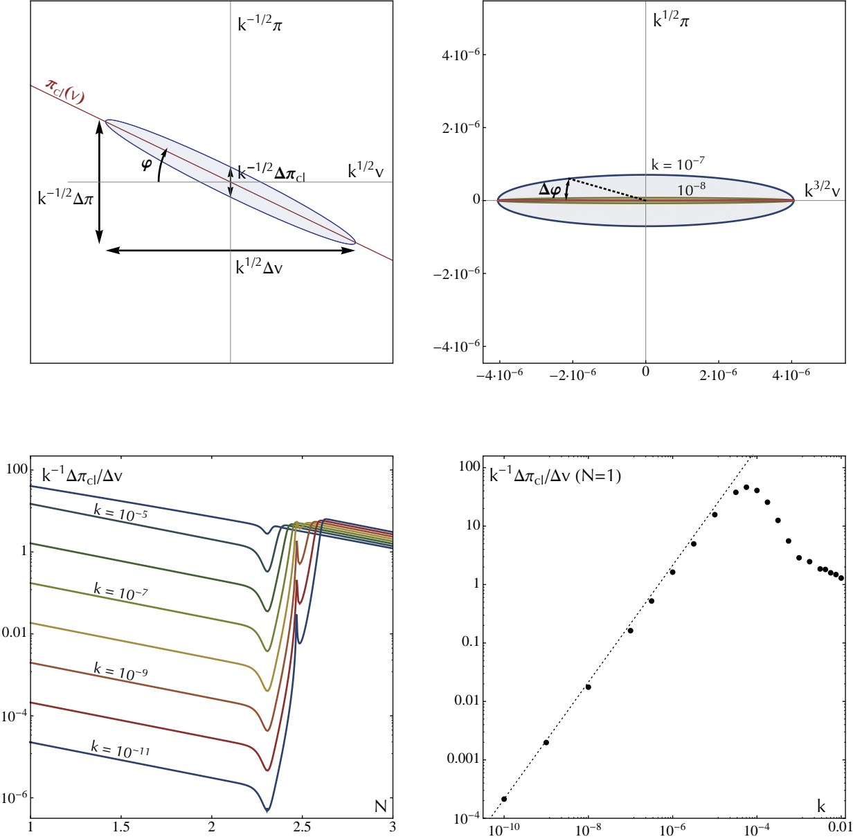
FIG. 4: Top, left panel: general shape of the Wigner ellipse for a gaussian state. Top, right panel: shape of the Wigner ellipses in the rescaled phase space at N = 1 for k = 10^{-7}, 10^{-8} and 10^{-9} . The plot shows that the dispersion of v scales very accurately as k^{-3/2} , while the dispersion of the temporal phase rapidly goes to zero: the k = 10^{-9} ellipse is barely distinguishable from a segment of the \pi = 0 line. Bottom panels: behavior of the temporal phase dispersion (III.25) as a function of N and at N = 1 for different values of k . The right panel indicates that \Delta\varphi \propto k (dotted line) for sufficiently small k .
