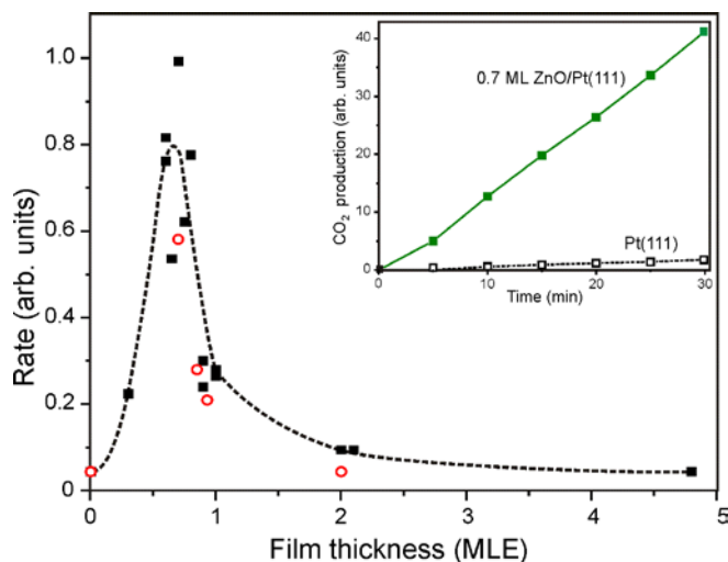
Figure 3. CO 2 production rate measured over ZnO films on Pt(111) as a function of the nominal film thickness (in MLE). Solid and open symbols show data for the films prepared using reactive Zn deposition at 85 and 300 K, respectively. Note that for the sub-monolayer films, the film thickness corresponds to the surface coverage as measured by CO titration of Pt(111). The inset shows kinetic curves for CO 2 production on the pure Pt(111) and 0.7 ML ZnO(0001) film. Reaction conditions: 10 mbar CO + 50 mbar O 2 , He balance to 1 bar; 450 K.
