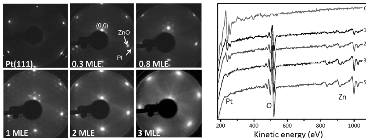
Figure 1. LEED patterns (at 60 eV, left panel) and Auger spectra (right panel) of ZnO films grown on Pt(111) at the nominal film thicknesses as indicated. Monolayer equivalent (MLE) values are shown to the right of the Auger spectra.
