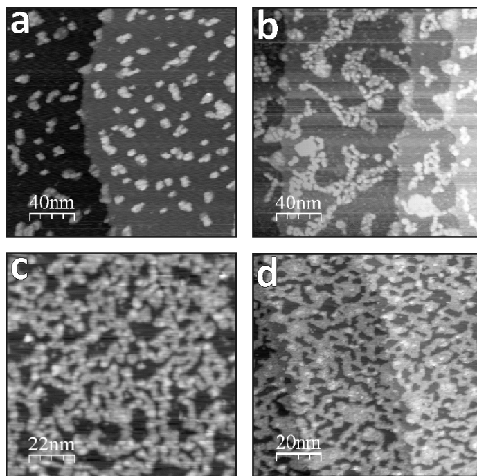
Figure 5. STM images of the “reacted” ZnO films at 0.25 (a), 0.55 (b), 0.8 (c) and 1.2 MLE (d) film thicknesses.
