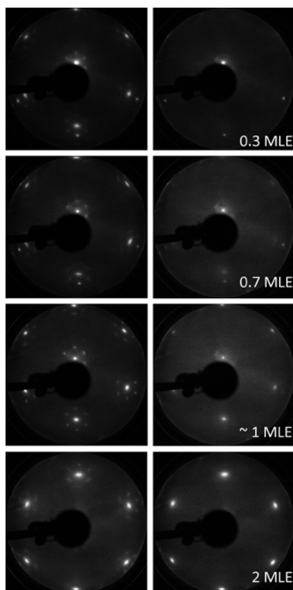
Figure 4. LEED patterns (60 eV) of the ZnO films on Pt(111) before (left panel) and after (right panel) the reaction. The film thickness is indicated.
