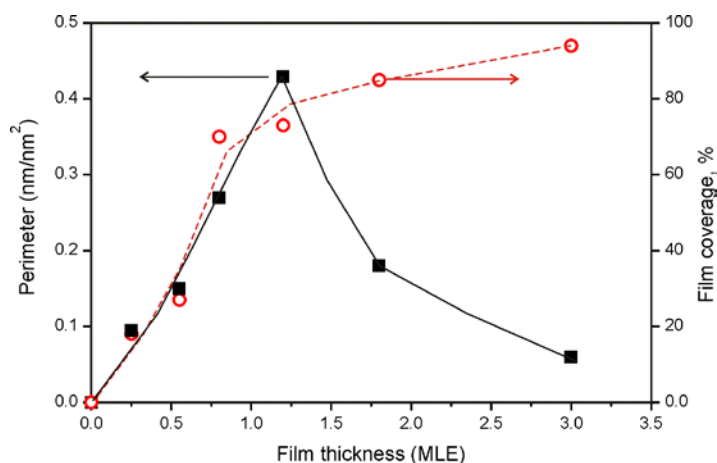
Figure 6. The perimeter of oxide/metal boundary and the film coverage measured by STM on the “reacted” samples as a function of the nominal film thickness measured on the same samples before the reaction (10 mbar CO + 50 mbar O 2 , He balance; 450 K; 10 min).
