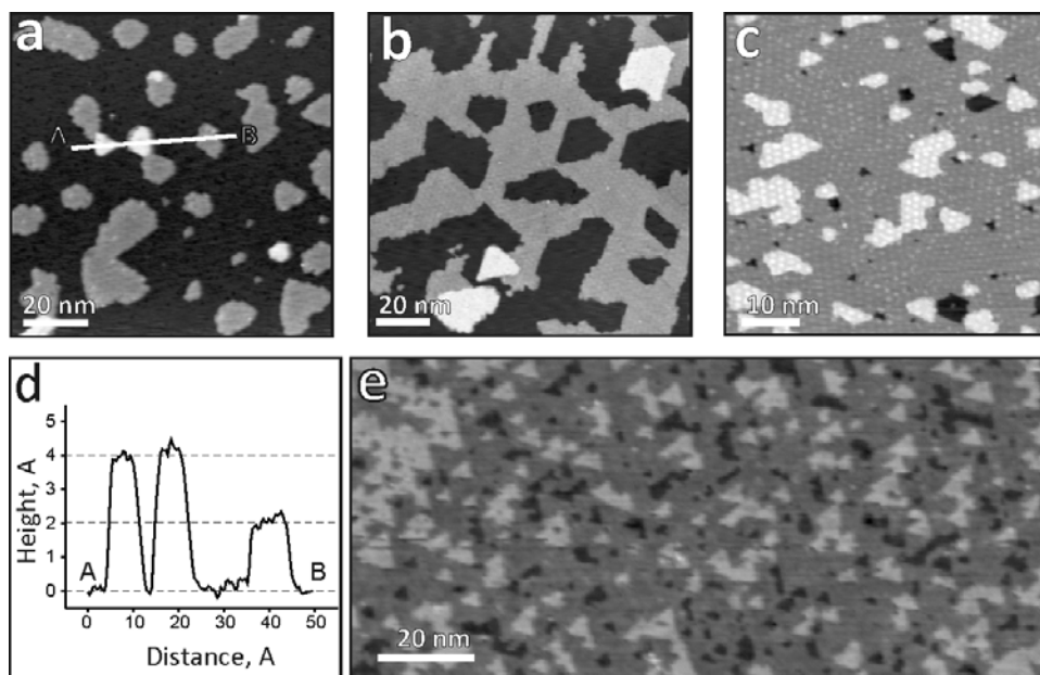
Figure 2. STM images of the “as prepared” ZnO films on Pt(111) at 0.25 (a), 0.55 (b), 1.2 (c) and 4 MLE (e) coverages. Figure (d) shows a profile scan along the A-B line marked in (a).
