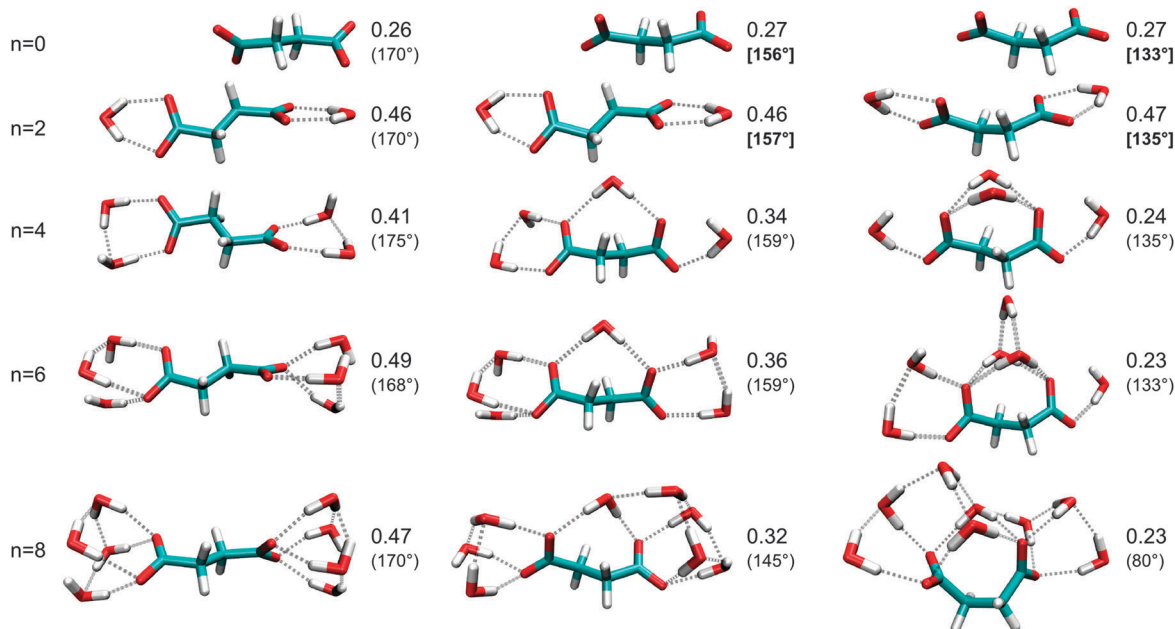
Fig. 5 Normalized intensities I_S / (I_S + I_A) for different configurations of the succinic acid dianion containing 0 (left), 1 (center), or 2 (right) water molecules bound to both carboxylates (bridging water molecules). The C-C-C dihedral is given in parentheses. In cases where bridging water molecules are not available ( n = 0 and n = 2 ), the structures have been optimized under a constrained C-C-C dihedral (boldface value in brackets) that is typical for a cluster with 1 (center) or 2 (right) bridging water molecules.
