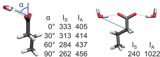
Fig. 6 Intensities I_S and I_A ( \text{km mol}^{-1} ) of the microsolvated butanoic acid anion ( in vacuo I_S and I_A are 291 and 554 \text{km mol}^{-1} , respectively). To achieve different hydrogen-bond orientations, the water oxygen positions were constrained during optimization by fixing the angle \alpha (left) or the C–O distance (right).
