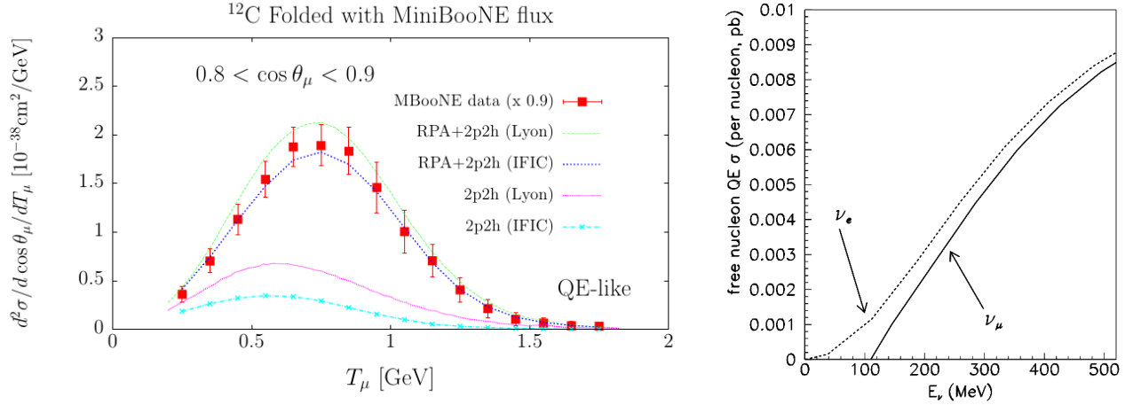
Figure 1: (left) MiniBooNE flux averaged CCQE-like cross section normalised per neutron with experimental points rescaled by 0.9. \cos\theta_\mu \in (0.8, 0.9) . Predictions from two theoretical models are compared and contributions from np-nh mechanism are also shown separately. (right) The total charged-current quasi-elastic cross-section for \nu_\mu and \nu_e neutrinos.
