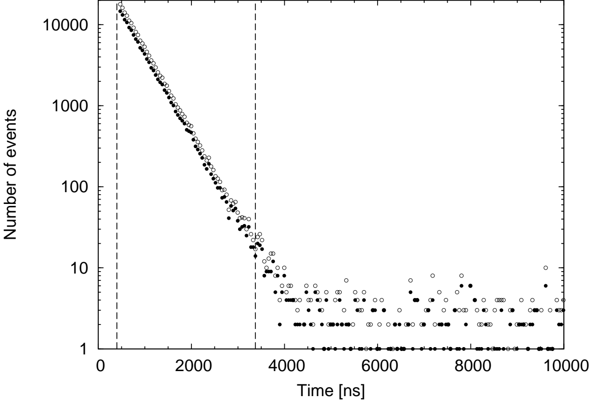
FIG. 5. Data from the first ^{212}\text{Po} source with 1000 bins between 400 and 48000 ns are shown up to 10000 ns. Number of TCE's as a function of the time difference t between the first and the second decay. Filled (open) dots show data with (without) the energy cuts reported in the text. Vertical lines delimit a seven-lifetime window.
