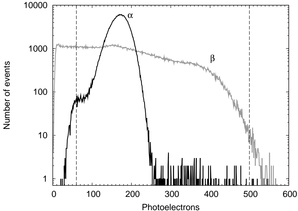
FIG. 3. Energy spectrum for the prompt (candidate \beta decay of ^{212}\text{Bi} , gray histogram) and delayed event (candidate \alpha decay of ^{212}\text{Po} , black histogram) of TCE from the second ^{212}\text{Po} source. Vertical dashed lines delimit the energy cuts used in the analysis for the \beta candidate; no cuts were used for the second event.
