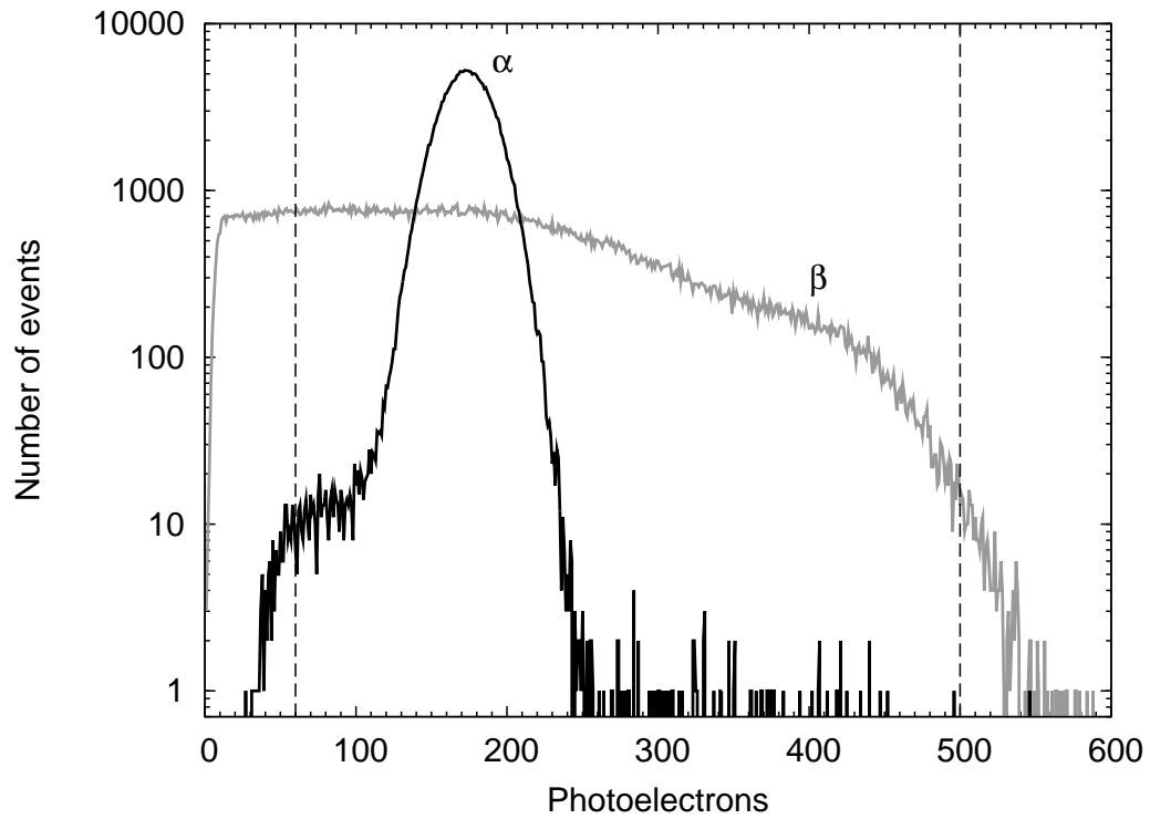
FIG. 2. Energy spectrum for the prompt (candidate \beta decay of ^{212}\text{Bi} , gray histogram) and delayed event (candidate \alpha decay of ^{212}\text{Po} , black histogram) of TCE from the first source. Vertical dashed lines delimit the energy cuts used in the analysis for the \beta candidate; no cuts were used for the second event.
