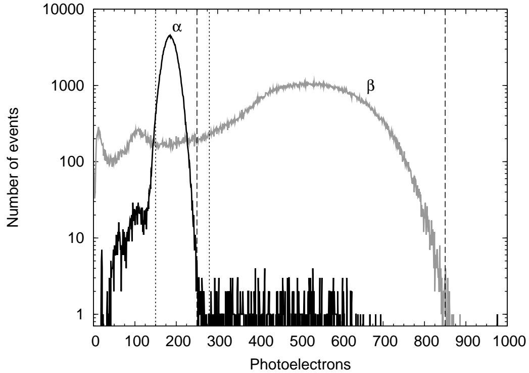
FIG. 1. Energy spectrum for the prompt (candidate \beta decay of ^{214}\text{Bi} , gray histogram) and delayed event (candidate \alpha decay of ^{214}\text{Po} , black histogram) of TCE. Vertical dashed (dotted) lines delimit energy cuts for the \beta ( \alpha ) candidates used in the analysis.
