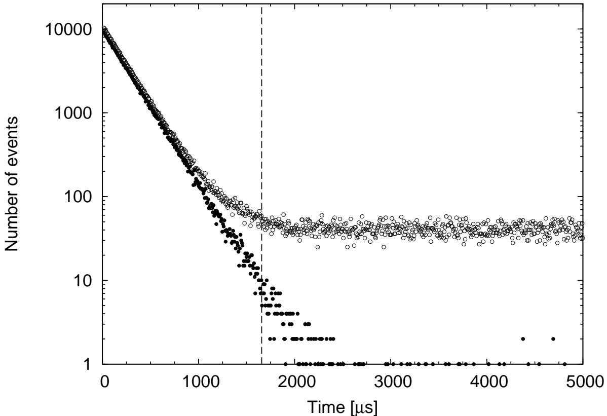
FIG. 4. Data from the ^{214}\text{Po} source with 1000 bins between 5 and 7605 \mu\text{s} are shown up to 5000 \mu\text{s} . Number of TCE's as a function of the time difference t between the first and the second decay. Filled (open) dots show data with (without) the energy cuts reported in the text. Vertical lines delimit a seven-lifetime window.
