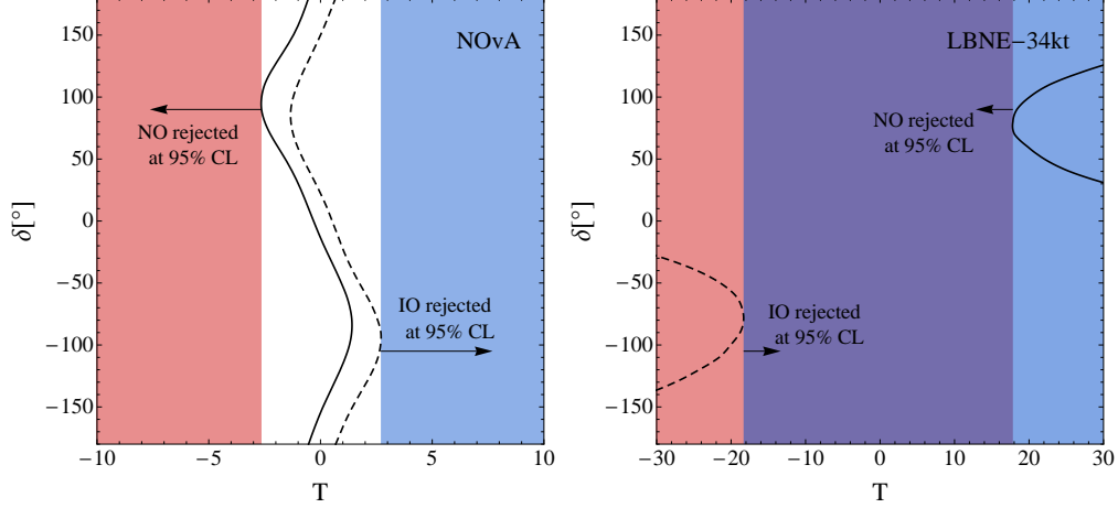
FIG. 8: The critical value T_c corresponding to 95% confidence level as a function of the CP-violating phase \delta for \text{NO}\nu\text{A} (left panel) and \text{LBNE-34 kt} (right panel). The solid (dashed) lines correspond to testing the normal (inverted) ordering. The red (blue) region corresponds to values of T which would reject all parameter values in the normal (inverted) ordering and thereby reject normal (inverted) ordering at 95% confidence level. In the white region, there are parameter values in both orderings which are allowed, while in the purple region none of the two orderings would be compatible with data at 95% CL.
