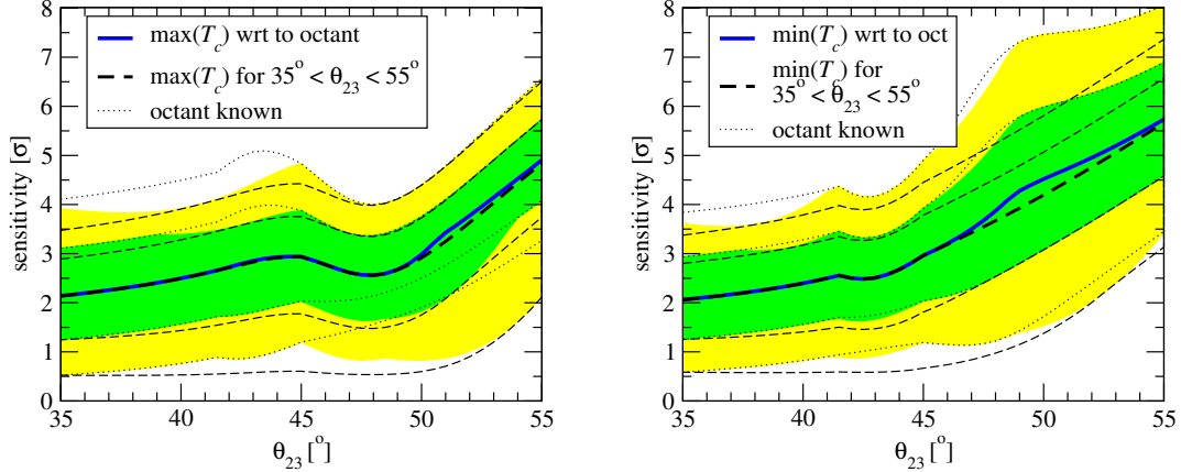
FIG. 5: Median sensitivity for PINGU after 3 years data taking as a function of the true value of \theta_{23} . Left (right) panel shows a test for NO (IO), which means that the true ordering is inverted (normal). For the thick black dashed curve we consider the range 35^\circ < \theta_{23} < 55^\circ for the true value of \theta_{23} when calculating the critical value for the test statistic ( T_c^\alpha ), and the thin dashed curves indicate the corresponding 68.27% and 95.45% probability ranges of obtained rejection significances. For the blue solid curve and the corresponding green (68.27%) and yellow (95.45%) probability bands we assume that \theta_{23} is known up to its octant when calculating T_c^\alpha . The dotted curves show the 68.27% and 95.45% probability ranges assuming that \theta_{23} including its octant is known (simple hypothesis test).
