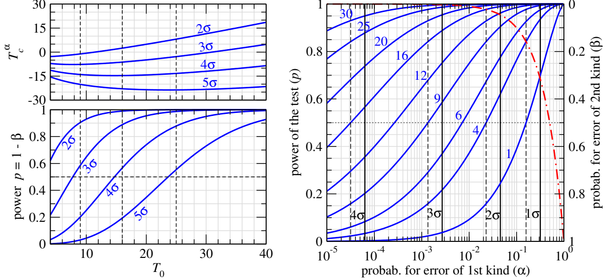
FIG. 2: Gaussian approximation for the test statistics T . Left upper panel: critical values for rejecting normal ordering as a function of T_0 , see Eq. (13), for different values of \alpha as labeled in the plot. Left lower panel: power of the test as a function of T_0 for different values of \alpha , see Eq. (14). Right panel: power of the test (left vertical axis) and the probability for an error of the second kind (right vertical axis) versus the CL ( 1 - \alpha ) for rejecting a given mass ordering for different values of T_0 as labeled in the plot. The vertical lines indicate the number of standard deviations, where we have used our standard convention Eq. (2) based on a 2-sided Gaussian for the solid lines and Eq. (3) based on a 1-sided Gaussian limit for the dashed lines. The dash-dotted red curve indicates \alpha = \beta , which follows in the Gaussian case from the condition T_c^{\text{NO}} = T_c^{\text{IO}} .
