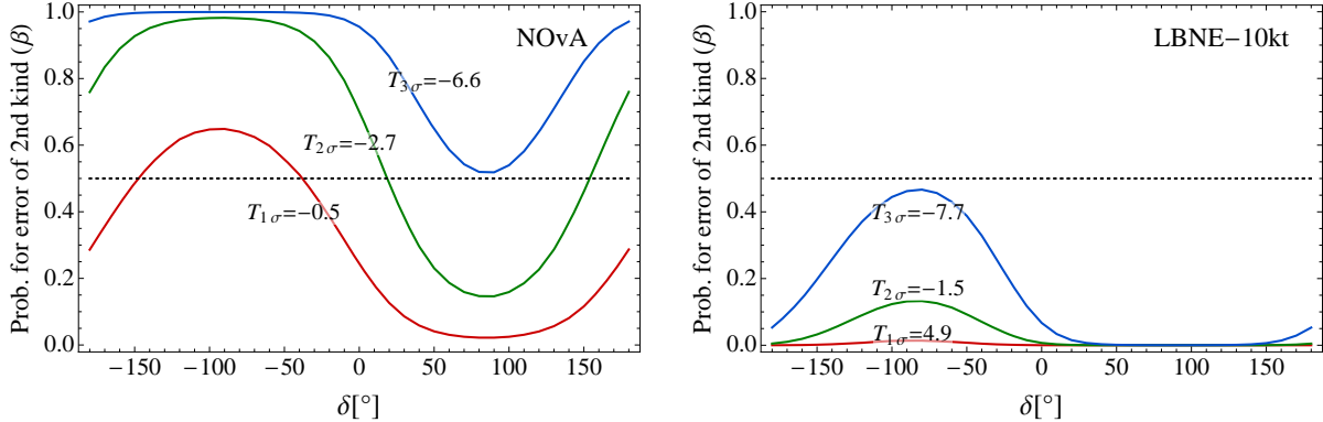
FIG. 9: Probability of accepting normal ordering if inverted ordering is true ( i.e. , error of the second kind) as a function of the true \delta in IO for the NO \nu A (left panel) and LBNE-10 kt (right panel) experiments. The different curves correspond to tests at 1\sigma , 2\sigma , 3\sigma confidence level, as labeled in the plot. Furthermore the corresponding critical values T_c^\alpha are given. The horizontal dotted lines indicate the median experiment, \beta = 0.5 .
