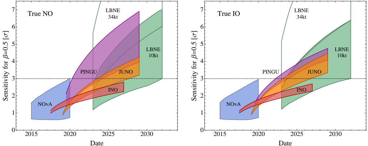
FIG. 11: The left (right) panel shows the median sensitivity in number of sigmas for rejecting the IO (NO) if the NO (IO) is true for different facilities as a function of the date. The width of the bands correspond to different true values of the CP phase \delta for \text{NO}\nu\text{A} and LBNE, different true values of \theta_{23} between 40^\circ and 50^\circ for INO and PINGU, and energy resolution between 3\%\sqrt{1 \text{ MeV}/E} and 3.5\%\sqrt{1 \text{ MeV}/E} for JUNO.
