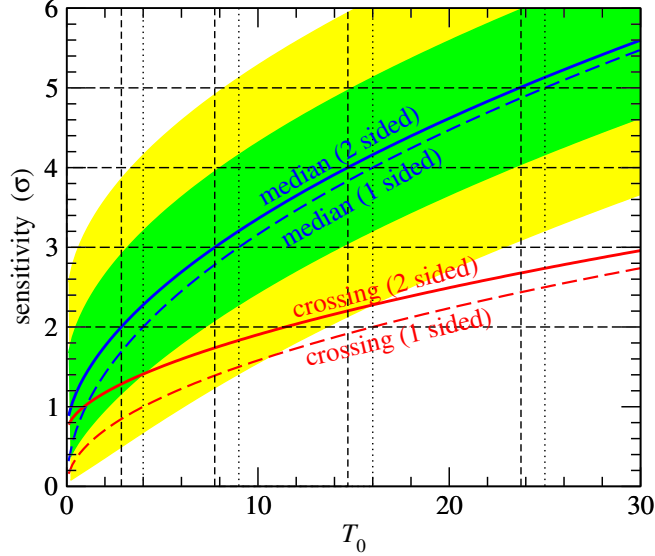
FIG. 3: Median sensitivity ( \beta = 0.5 ) as a function of T_0 , see Eq. (16). The curves labeled “crossing” show the sensitivity corresponding to the condition T_c^{\text{NO}} = T_c^{\text{IO}} according to Eq. (17). The solid curves use the 2-sided Gaussian to convert \alpha into n\sigma , Eq. (2), whereas the dashed curves are based on the 1-sided test, Eq. (3). The latter correspond to the “standard sensitivity” of n = \sqrt{T_0} and n = \sqrt{T_0}/2 for the crossing sensitivity. The green (yellow) band indicates the range of \sigma with which a false null hypothesis will be rejected in 68.27% (95.45%) of experiments with the corresponding T_0 .
