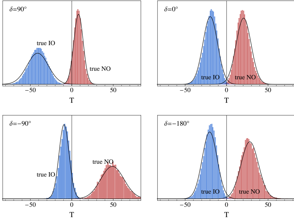
FIG. 7: The simulated distributions of the test statistic T in the LBNE-10 kt experiment for different true values of \delta , as indicated by the labels. The red (blue) distributions assume a true normal (inverted) ordering. Solid curves indicate the Gaussian approximation for T from Eq. (12).
