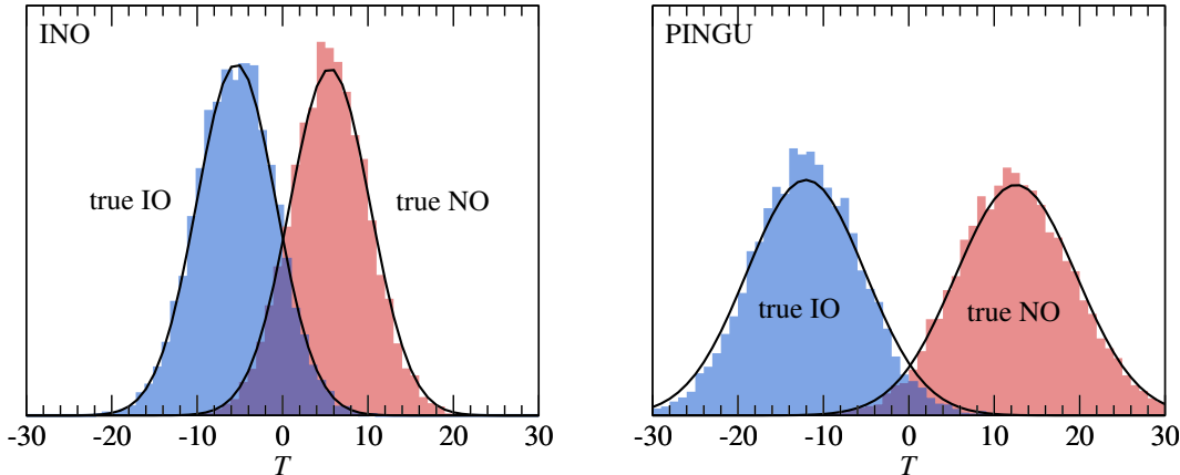
FIG. 4: Histograms show the simulated distributions of the test statistic T in the INO (left) and PINGU (right) experiments. We use our default setups as defined in Tab. II and assume \theta_{23} = 45^\circ . Solid curves show the Gaussian approximation from Eq. (12)
