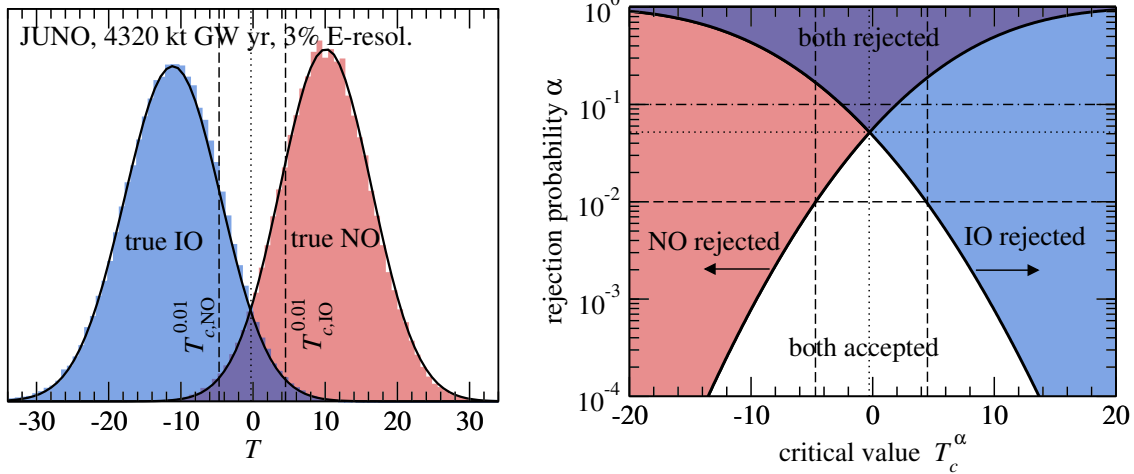
FIG. 1: Left: Distribution of the test statistic T for our default configuration of the JUNO reactor experiment discussed in Sec. IV A. Histograms show the results of the MC simulation based on 10^5 simulated experiments and black curves correspond to the Gaussian approximation discussed in Sec. III. Right: The value of \alpha as a function of the critical value T_c^\alpha required for rejecting inverted (blue) and normal (red) ordering for the JUNO reactor experiment. In the purple region both mass orderings are rejected at the CL (1 - \alpha) , in the white region both orderings are consistent with data at the CL (1 - \alpha) . The dashed lines in both panels indicate T_c^\alpha for \alpha = 0.01 for both orderings. The dotted lines indicate the crossing point T_c^{\text{NO}} = T_c^{\text{IO}} . The dot-dashed line in the right panel shows an example (for \alpha = 0.1 ) in which T_{c,\text{IO}}^\alpha < T_{c,\text{NO}}^\alpha .
