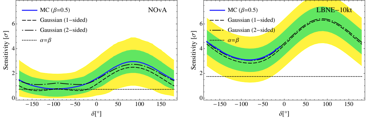
FIG. 10: Comparison of the median sensitivities based on a full MC simulation to the results based on the Gaussian approximation Eq. (21). The number of sigmas at which the normal mass ordering can be rejected with a probability of 50% are shown as a function of the true value of \delta in the inverted ordering for \text{NO}\nu\text{A} (left panel) and \text{LBNE-10 kt} (right panel). The results obtained by a full MC simulation are shown by the solid thick lines. The results for the Gaussian approximation are shown by using a 2-sided (dot-dashed) and 1-sided (dashed) Gaussian probability to convert \alpha into number of standard deviations. The 1-sided version corresponds to n = \sqrt{T_0} , i.e. , the “standard sensitivity”. The dotted horizontal lines show the sensitivity corresponding to the “crossing point” defined in Sec. II, which guarantees that \beta \lesssim \alpha . The missing points in the curve for the MC results for \text{LBNE-10 kt} require a number of simulations above 4 \times 10^5 (per value of \delta ) and are therefore not computed here. The green (yellow) band shows the range of \sigma with which a false null hypothesis will be rejected in 68.27% and 95.45% of the experiments.
