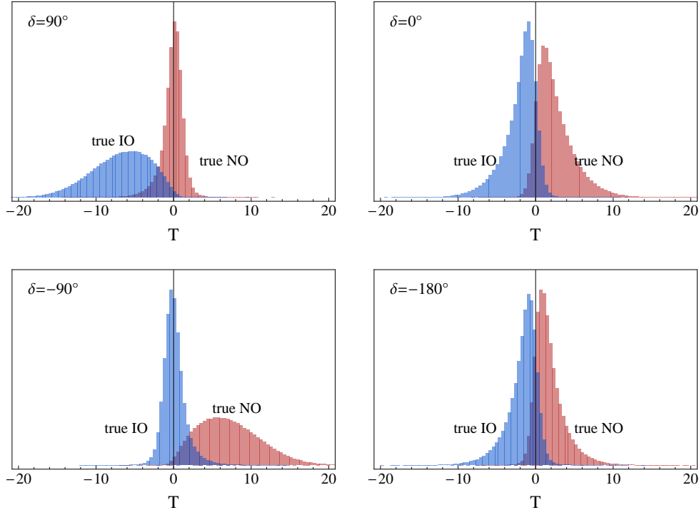
FIG. 6: The simulated distributions of the test statistic T in the \text{NO}\nu\text{A} experiment for different true values of \delta , as indicated by the labels. The red (blue) distributions assume a true normal (inverted) ordering.
