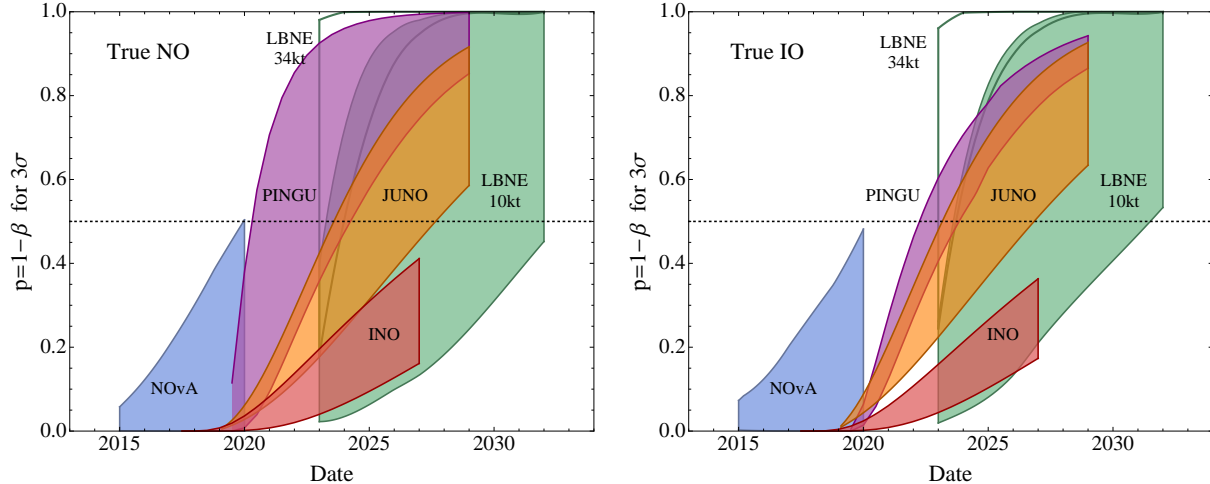
FIG. 12: Probability that the wrong ordering can be rejected at 3\sigma (99.73% CL) for a true NO (left) and IO (right) for different facilities as a function of the date. The width of the bands has the same origin as in Fig. 11. The dotted horizontal line indicates the median experiment ( \beta = 0.5 ).
