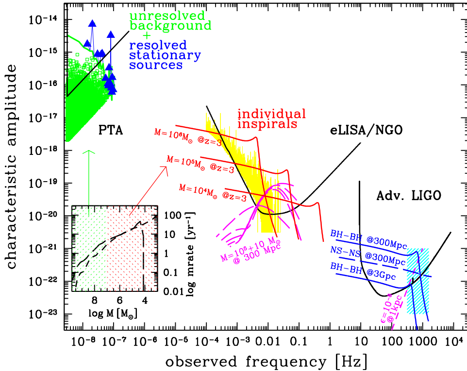
Fig. 1 Summary of the GW landscape discussed in the text. Black solid curves are detector sensitivities as labeled in the figure. For the PTA sensitivity curve we considered an SKA-like scenario in which 500 MSPs are monitored for 10 yrs at 50ns precision. In the Adv. in the LIGO band, the blue curves represent inspirals of compact stellar mass binaries [14], the dashed magenta line marks the expected strain for rapidly spinning NSs [25], and the shaded cyan box identifies the area where burst signals from collapsing SNe are expected [19]. In the eLISA/NGO band, the red curves represent merging MBH binaries at cosmological distances, the dashed-magenta line is a typical eccentric EMRI at z = 0.1 (only the first 5 harmonics are shown) and the jagged yellow curve is the overall signal from a galactic population of WD-WD binaries. In the PTA band, the total signal (green solid line) is given by an incoherent superposition of individual MBH binaries (green dots); the brightest sources can be individually resolved (blue lines and triangles). The lower-left inset shows the inferred cosmological merger rate of MBH binaries as a function of mass for two specific models [26]. eLISA/NGO will probe the low mass part of the distribution (red shade) by detecting individual merging systems, whereas PTA will probe the high mass end (green shade) of the mass function by collecting signals from very massive systems in their inspiral phase.
