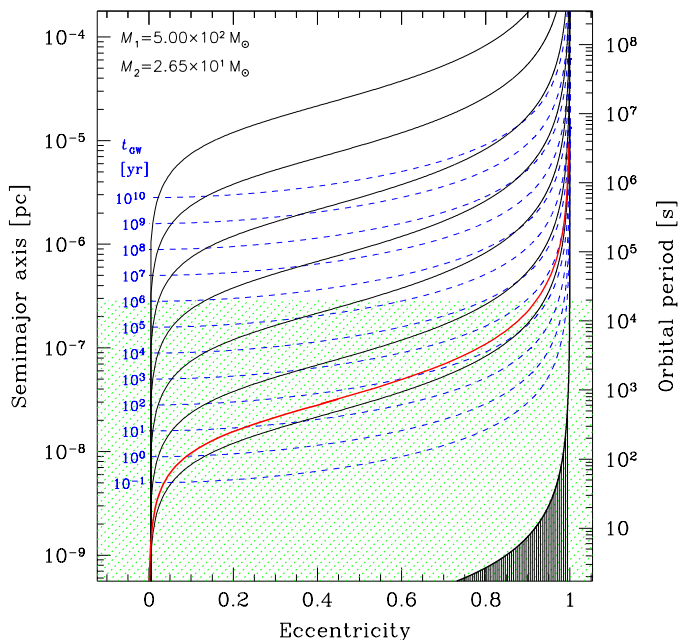
Fig. 4. Inspiral of the SBH into the IMBH from the top to the bottom and from the left to the right in the eccentricity–semi-major axis plane. The red, solid curve starting at a very eccentric orbit shows the results of the NBODY simulation. The dashed, green region corresponds to the band of a LISA-like mission. Dashed, blue curves correspond to the trajectories due only to the emission of GWs in the Peters & Mathews (1963) approximation. We also plot the corresponding merger timescales in the same approximation in dashed, blue lines starting at 10^{10} years, and in solid, black lines the corresponding trajectories for evolution by GW emission Peters (1964) approximation. The black-shaded region on the right corresponds to the last stable circular orbit. Since the binary starts at a very high eccentricity, it basically follows one of the solid black lines, because it merges quickly and does not interact with other stars in the system.
