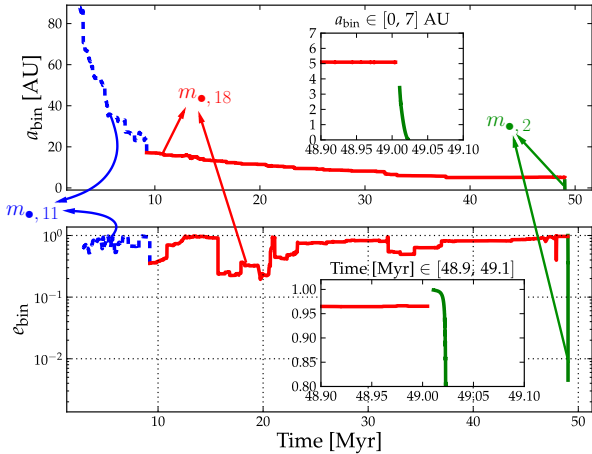
Fig. 1. Evolution of the semi-major axis and eccentricity of the different three binaries formed with the IMBH. Shortly after the beginning of the simulation, the IMBH builds a binary with the SBH with the 11th most massive mass, m_{\bullet, 11} . This corresponds to the first part of the curve (dashed blue curve). Later there is an interaction which leads to a companion exchange for the binary, the SBH with the 18th most massive mass, m_{\bullet, 18} . This binary lives for about 40 Myr. We can see that the two first binaries have phases of very high eccentricity, e_{\text{bin}} \sim 1 , but not high enough to lead to a coalescence. The jumps in e_{\text{bin}} indicate that the IMBH-SBH is still in a regime in which interactions with other stars play an important role. The system shrinks further and further until there is a three-body interaction. The binary is unbound and for a short period of time the IMBH has no companion, as indicated in the zoom-in subplots embedded in both, the upper and lower panels. Then the final binary forms, with the second most massive SBH. This binary is very hard and quickly losses energy via GWs radiation, which very efficiently leads to circularization and the final merger.
