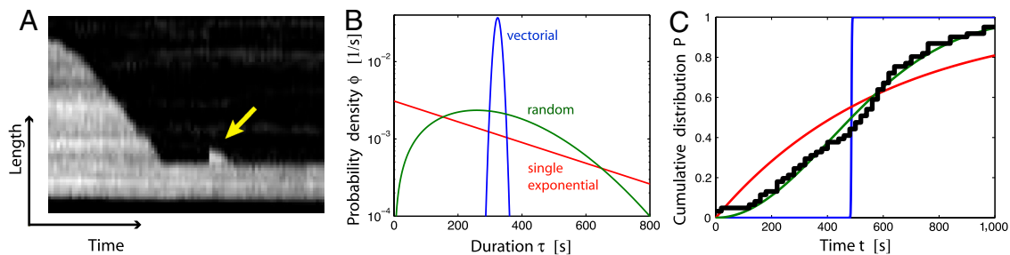
Fig. 2. Interruptions of depolymerization arise from local transitions at random filament sites. (A) After the interruption of initial depolymerization, we switched first to polymerization conditions for a short time period and then back to depolymerization conditions. The depolymerizing filament displayed a second interruption at precisely the same position, at which the first interruption had occurred, see small “shark fin” indicated by the arrow. (B) Alternative probability densities for the duration \tau of the initial shrinking phase (semilogarithmic plot). The red curve represents a single exponential distribution, the blue one corresponds to a putative vectorial process, and the green one to random protomer transitions. (C) Comparison of theoretical and experimental results for the cumulative distribution, i.e., the probability that the interruption occurs at any time prior to time t . The colored lines, which represent the same mechanisms as in (B), were obtained by least-square-fitting to the experimental data (black) using the transition rate \omega as the only fit parameter. The green line for random transitions leads to the rate \omega \approx 10^{-6}/s . The data were obtained from 61 filaments, polymerized from MgATP-actin using the microfluidics setup in Fig. 1C.
