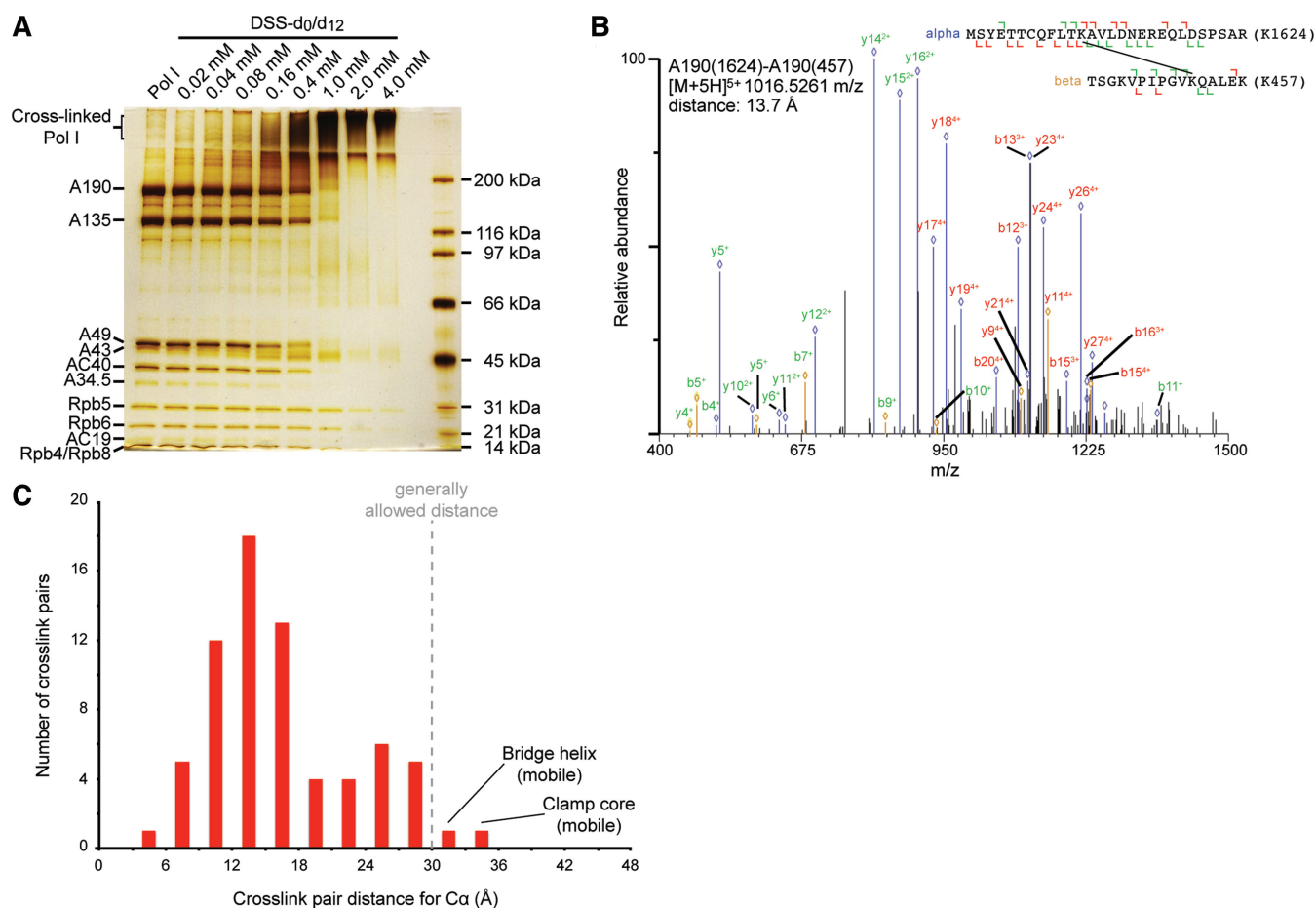
Figure 2. Crosslinking-MS analysis of Pol I. (A) SDS-PAGE analysis of Pol I crosslinked with different concentrations of DSS. (B) Fragmentation spectrum of a crosslinked peptide. The linkage site A190 K1624-A190 K457 was observed in the crosslinked peptide MSYETTCQLTK(xl)AVLDNEREQLDSPSAR/TSGKVPVIGVK(xl)QALEK (m/z 1016.5261, 5+; 'xl' denotes the crosslinked lysine). Extensive ion series for both peptides are observed in the fragmentation spectrum providing high confidence in the match. Peaks of the \alpha - and \beta -peptide are colored blue and ochre, respectively. Common ions are labeled in green, and crosslink ions are labeled in red. (C) C\alpha distance distribution for experimentally observed A-A linkage pairs within the Pol I 9-subunit core (subunits A190, A135, AC40, AC19, Rpb5, Rpb6, Rpb8, Rpb10 and Rpb12). The generally allowed distance between the C\alpha atoms of two crosslinked lysine residues of 30 Å is indicated by a dashed line. Observed crosslinks are in agreement with the homology model for the Pol I core as judged by analysis with the Pol II X-ray structure (PDB 1Y1V).
