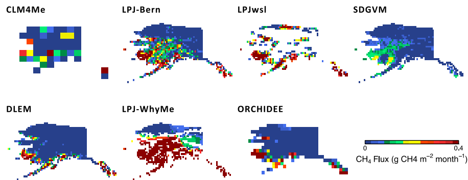
Fig. 4. Mean annual (2003) net \text{CH}_4 flux for Alaska. Model output was part of the WETCHIMP model intercomparison project.
