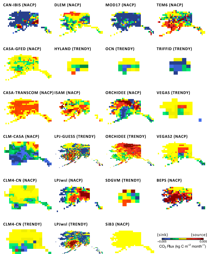
Fig. 2. Mean annual (2003) net CO 2 flux for Alaska. Model output was part of the TRENDY (common forcing) and NACP Regional (variable forcing) syntheses.
