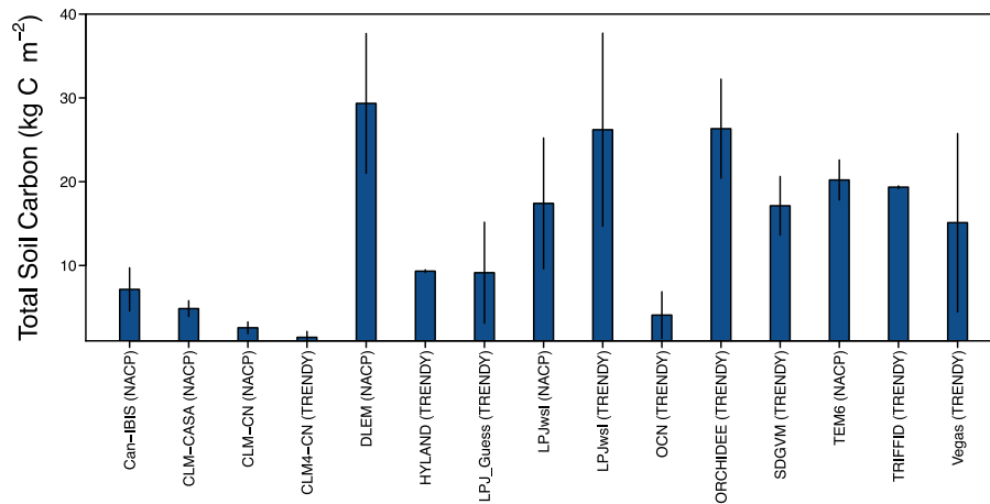
Fig. 6. Mean annual Alaskan Arctic total soil carbon with spatial standard deviations.
