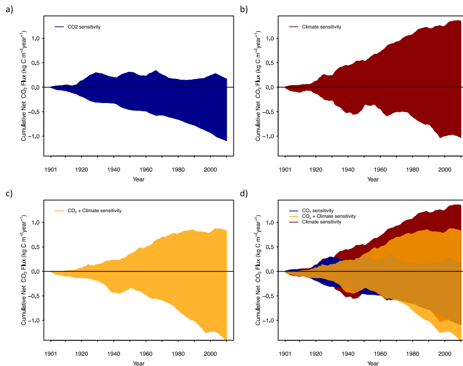
Fig. 10. Feedback/sensitivity analysis for the Alaskan Arctic showing the multi-model ( n = 9 ; TRENDY) standard deviation of net CO 2 flux accumulation over the 20th century for: (a) CO 2 fertilization alone ( \beta ); (b) climate impact alone ( \gamma ); (c) the combined impact of \beta and \gamma ; and, (d) all three feedbacks overlain for visual comparison.
