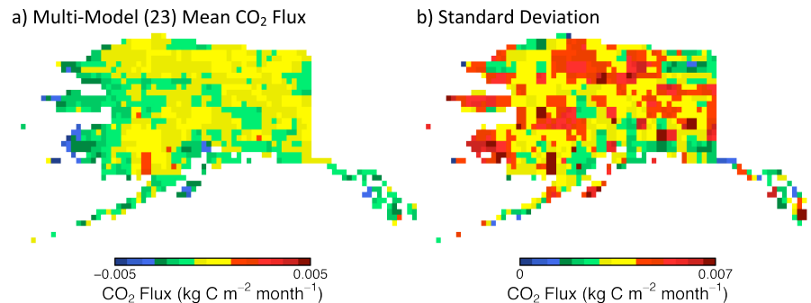
Fig. 3. NACP and TRENDY multi-model ( n = 23 ) net CO 2 flux for 2003 (a) mean, and (b) standard deviation.
