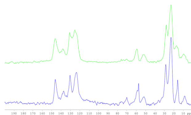
Figure 5 13 C CP-MAS NMR spectra of the hybrid SBA-NHC 2 (blue) and of the grafted SBA-NHC 4 (green).
