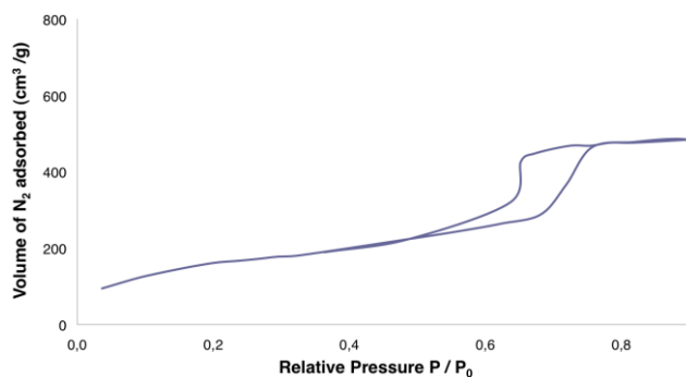
Figure 4 N 2 adsorption-desorption isotherm of the hybrid SBA-NHC 2 .
