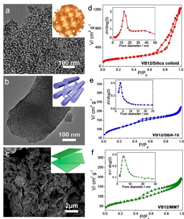
Figure 1. (a,b) TEM images and (c) SEM image of as-prepared C-N-Co catalysts: (a) VB12/Silica colloid, (b) VB12/SBA-15, and (c) VB12/MMT. Insets in (a-c) are the model illustration of the catalysts with various mesoporous structures. (d-f) N 2 sorption isotherms of these three C-N-Co catalysts. Insets show the pore size distribution from the BJH method of corresponding samples.
