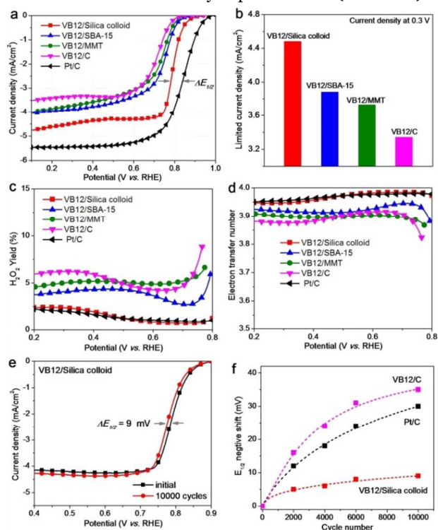
Figure 2. (a) ORR polarization plots of different C-N-Co catalysts. Electrode rotation speed, 1600 rpm; scan rate, 10 mV/s. (b) Limited current density of various C-N-Co catalysts at 0.3 V. (c) H 2 O 2 yield and (d) electron transfer number of different C-N-Co catalysts and Pt/C as functions of the electrode potential. (e) ORR polarization plots of VB12/Silica colloid before and after 10,000 potential cycles in O 2 -saturated electrolyte. (f) Negative shift of the half-wave potential ( E_{1/2} ) of VB12/Silica colloid, VB12/C, and Pt/C catalysts with the number of CV cycles under O 2 .
