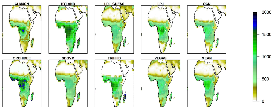
Fig. 4. Average Net Primary Productivity (NPP) for each DGVM and model mean over the period 1990–2009, units, \text{kg C m}^{-2} \text{ yr}^{-1} .
