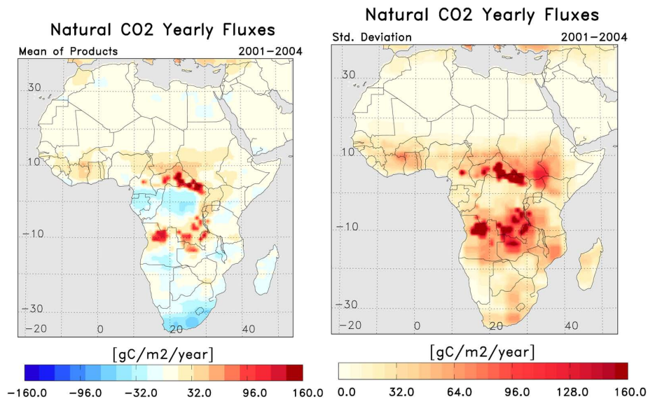
Fig. 3. (a) Distribution of mean CO 2 fluxes averaged across the five recent inversions analyzed. (b) shows the spread of the inversions (defined from the estimator of the standard deviation). Inversions have a different spatial resolution, and the fluxes have been interpolated on a common grid. Negative values are atmospheric CO 2 sinks ( http://www.carboscope.eu/ ).
