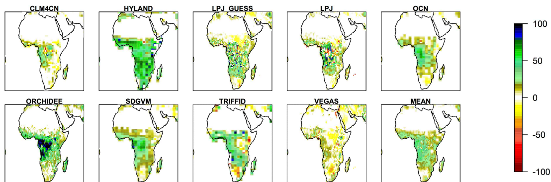
Fig. 5. Average Net Biome Productivity (NBP) for each DGVM and model mean over the period 1990–2009, units, \text{kg C m}^{-2} \text{yr}^{-1} .
