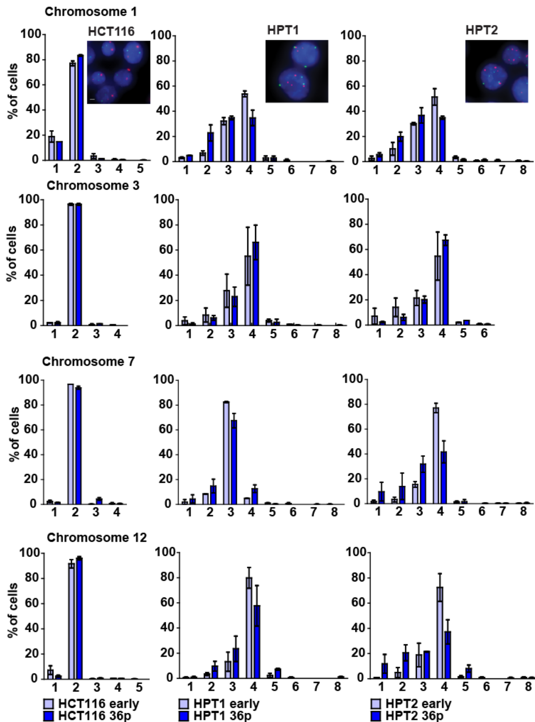
Figure 13. Chromosome numbers upon propagation in posttetraploid cells.
