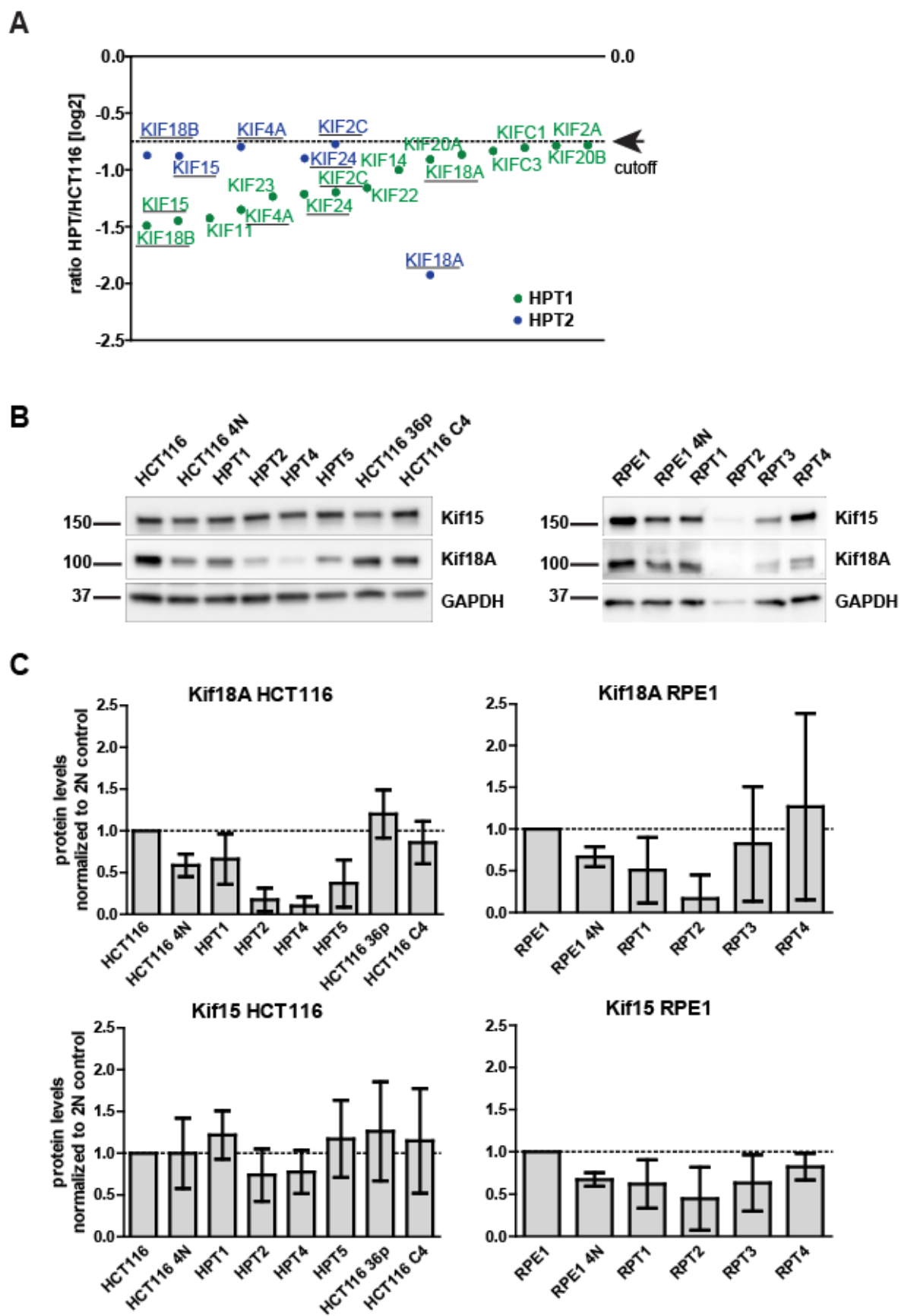
Figure 26. mRNA and protein level analysis of Kif15 and Kif18A in HCT116 and its derivatives.
