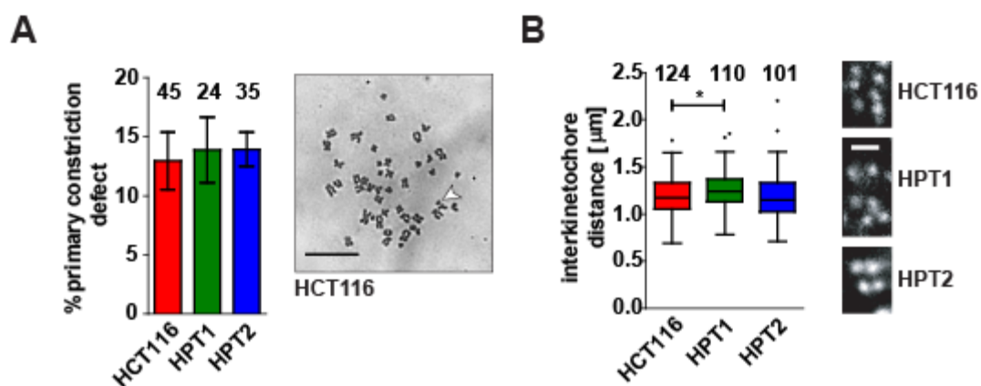
Figure 25. Sister chromatid cohesion in HCT116 and the posttetraploid cells.
