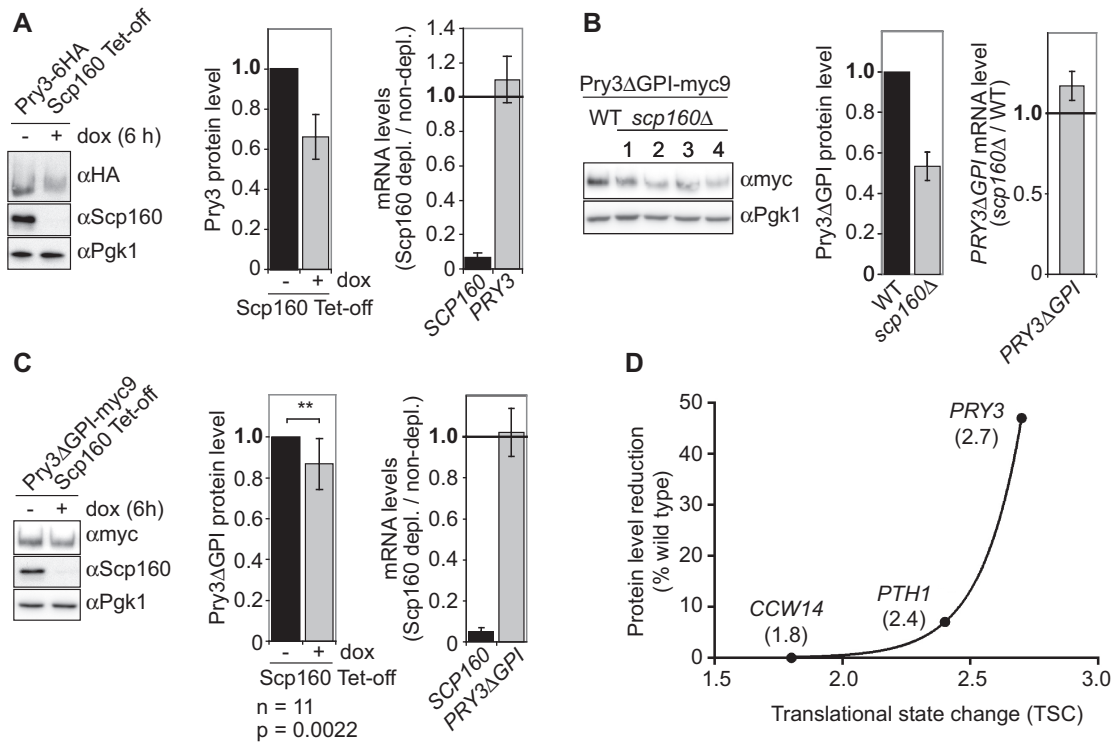
Figure 3. PRY3 protein levels are reduced on loss of Scp160p. (A) PRY3-6HA levels in Scp160-depleted cells. Whole cell extracts were prepared from strain RJY3498, 6 h after addition of 2 μg/ml doxycycline or after mock depletion. Left panel: equivalent total protein amounts were used for western blotting. Probing with anti-Scp160p antibody shows the efficient depletion of Scp160p, anti-HA antibody the reduction of PRY3-6HA protein levels on depletion of Scp160p and Pgk1 serves as loading control. One representative experiment is shown. Middle panel: quantification of four experiments performed as in the left panel. Right panel: RNA was prepared from the same samples and used for qRT-PCR as described in ‘Materials and Methods’ section. Relative PRY3 and SCP160 mRNA levels were calculated as signal ratio between Scp160p-depleted and non-depleted samples. All data are presented as mean ± standard deviation, n = 4 . (B) PRY3ΔGPI levels in scp160Δ cells. Whole cell extracts were prepared from yeast cells expressing PRY3ΔGPI-9myc and four independent clones of scp160Δ yeast cells expressing PRY3ΔGPI-9myc. Left panel: western blot of one representative experiment. Middle panel: quantification of three independent experiments carried out as in the left panel. Right panel: RNA was prepared from the same strains and used for qRT-PCR. Relative PRY3ΔGPI mRNA levels are represented as the signal ratio between scp160Δ and wild type (WT) background. (C) PRY3ΔGPI levels in Scp160p-depleted cells. Whole cell extracts were prepared 6 h after addition of 2 μg/ml doxycycline or after mock depletion. Left panel: representative western blot showing the efficient depletion of Scp160p (anti-Scp160p) and the reduction of PRY3ΔGPI-9myc protein levels on depletion of Scp160p (anti-myc). Pgk1 serves as loading control. Middle panel: quantification of n = 11 experiments performed as in the left panel. The decrease of the PRY3ΔGPI-9myc protein levels in the sample depleted for Scp160p is highly significant (Student’s t -test, P = 0.0022 ). Right panel: RNA was prepared from the same samples and used for qRT-PCR. Relative PRY3 and Scp160 mRNA levels were calculated as the signal ratio between Scp160p-depleted and non-depleted samples. All data are presented as mean ± standard deviation, n = 3 . (D) Polysome shift (TSC) and protein level reduction PRY3, PTH1 and CCW14 show pronounced non-linear correlation (Spearman’s r = 1.00 , P = 0.33 ). TSC values extracted from Supplementary Table S4 are indicated below targets for enhanced clarity.
