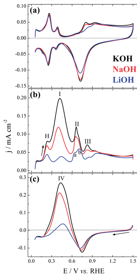
Fig. 1 Voltammetric characterization of the platinum electrode in (a) 0.1 M OH - (M = K, Na, Li); and after addition of 0.1 M HCOO - along the (b) positive-, and (c) negative-going sweep. dE/dt = 50 mV s -1 .
